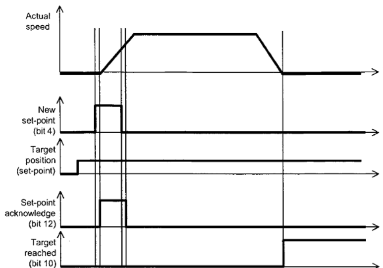
Figure 7.3: Adjustment of the position set-point (Source: IEC 61800-7-201)
