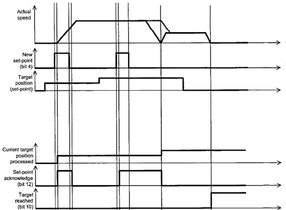
Figure 7.5: Set of set-point method (Source: IEC 61800-7-201)
