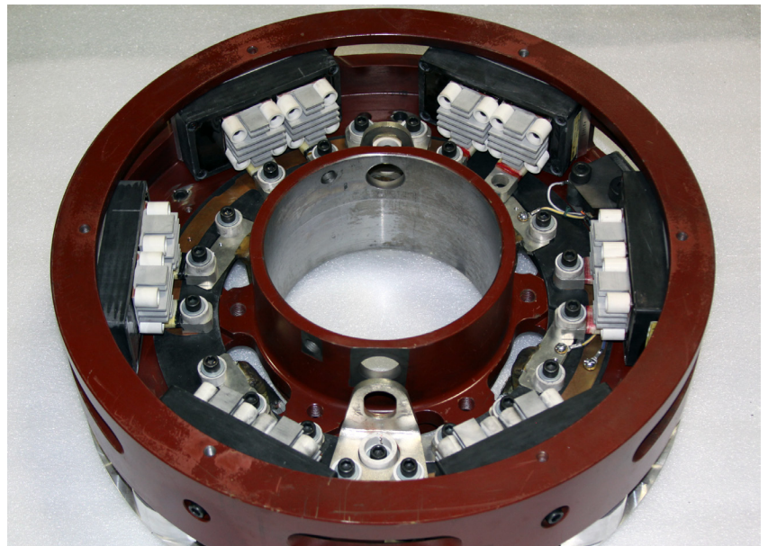
Complete Diode Wheel
