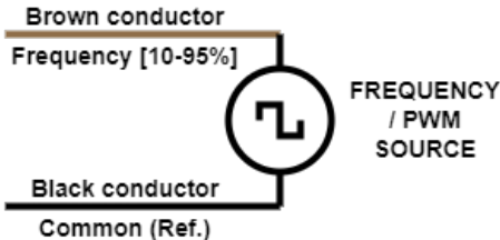
Figure 12 - Frequency input
