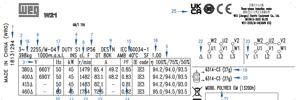
Figure 7 -Nameplate
