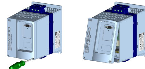
(c) Remove the screws from the front cover (c) Retire los tornillos de la tapa frontal (c) Retire os parafusos da tampa frontal
