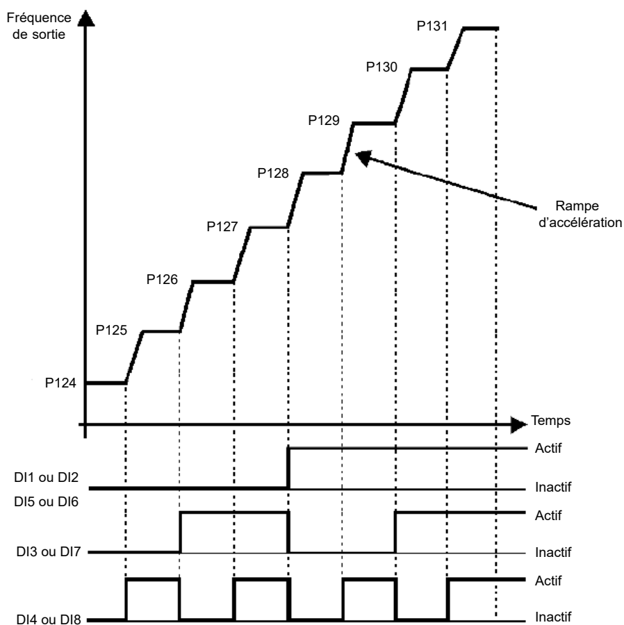
Figure 7.3 : Multispeed
