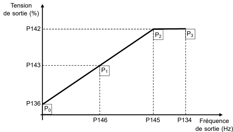
Figure 8.13 : Courbe V/f
