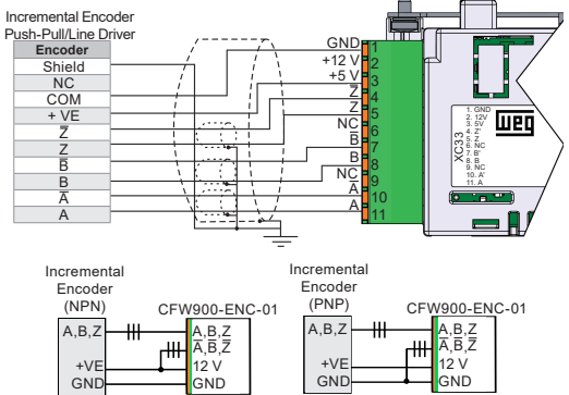
Figure A.2: Example of incremental encoder connection with push-pull or differential line driver, NPN and PNP outputs to the CFW900-ENC-01
