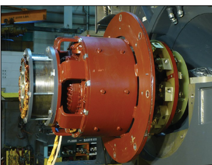
Rotating Armature and Rectifiers
