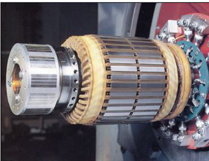
Stationary Exciter Field
