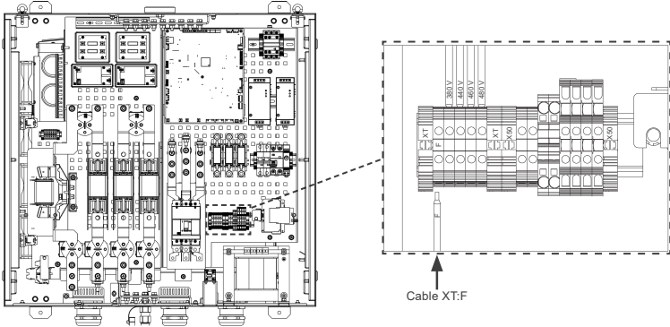
Figure 5.3: Setting the supply voltage
