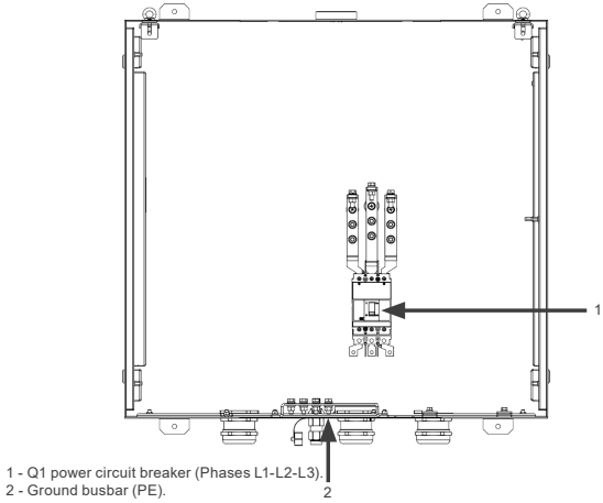
Figure 5.2: Power cable connections - Phases (L1-L2-L3) and ground (PE)
