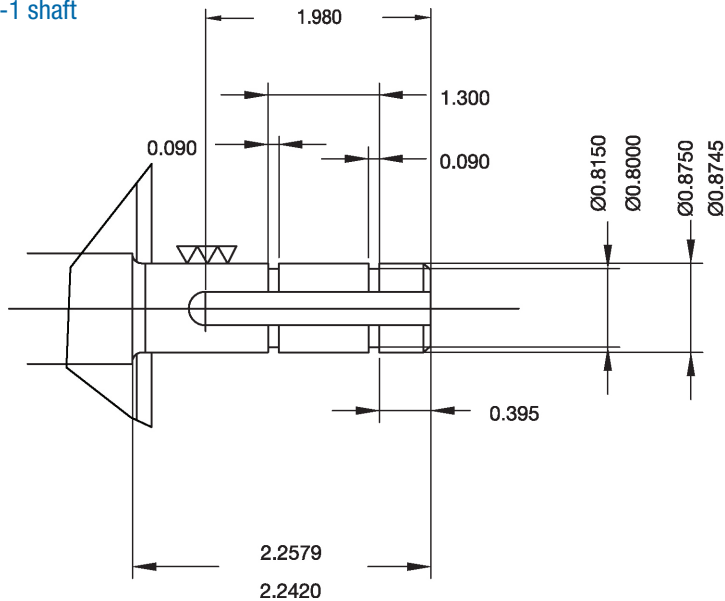
Type -1 shaft
