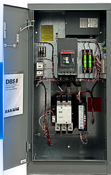
Original RAM DBS 400 HP State Starter
