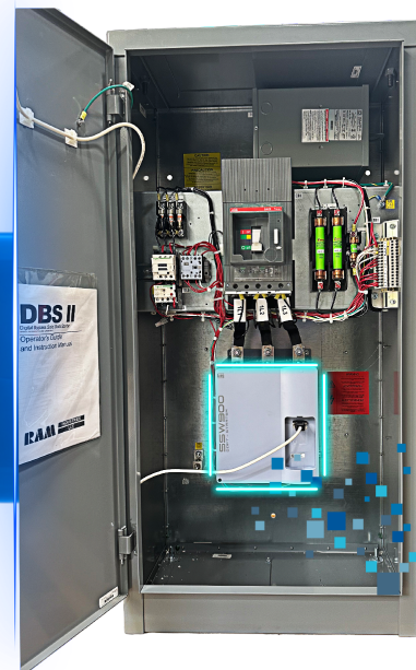
Retrofitted 400 HP Soft Starter with WEG SSW900
