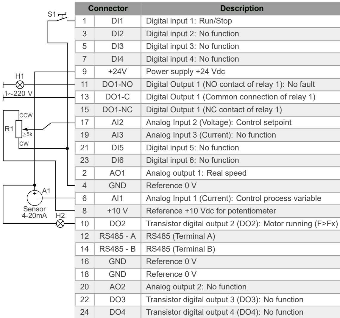
Figure 4.4: Signals on connector of the CFW500-IOAD plug-in module for setpoint via analog input
