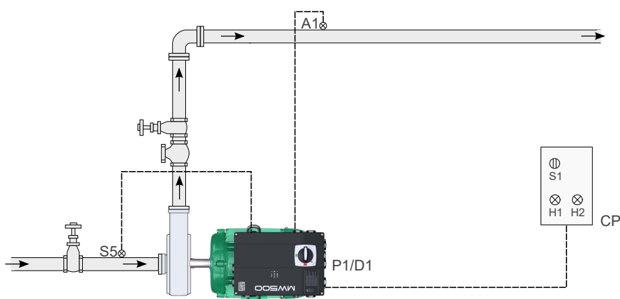
Figure 4.9: Pump Genius Simplex application and pump protection via external sensor in the digital input DI1
