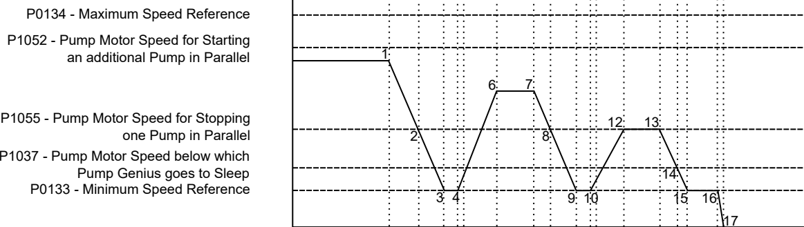
Figure 4.26: Operation description of the Pump Genius Multiplex with three pumps in parallel
