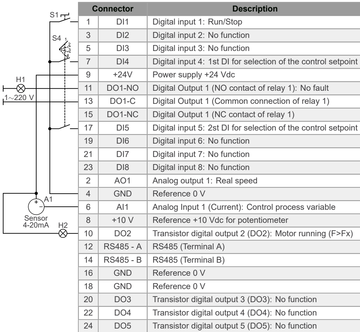
Figure 4.6: Signals on connector of the CFW500-IOD plug-in module for setpoint via logic combination of Digital Inputs
