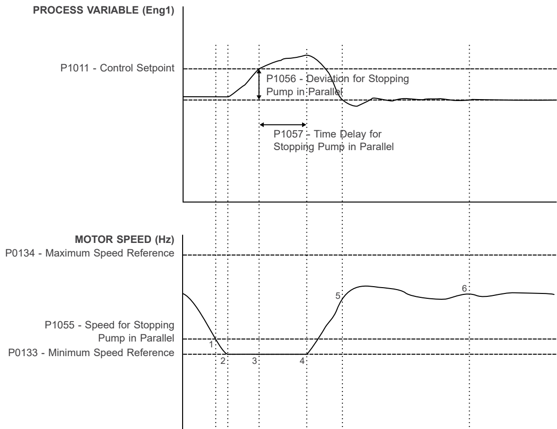
Figure 5.6: Pump Genius Multiplex operation for stop one pump in parallel
