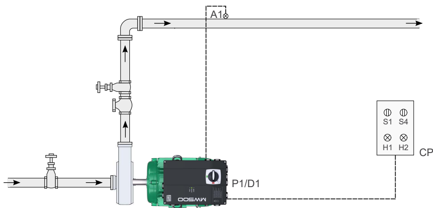
Figure 4.5: Pump Genius Simplex application and control setpoint via combination of the digital inputs DI4 and DI5
