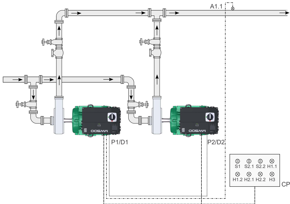
Figure 4.15: Pump Genius Multiplex application with two pumps in parallel and RS485 communication interface
