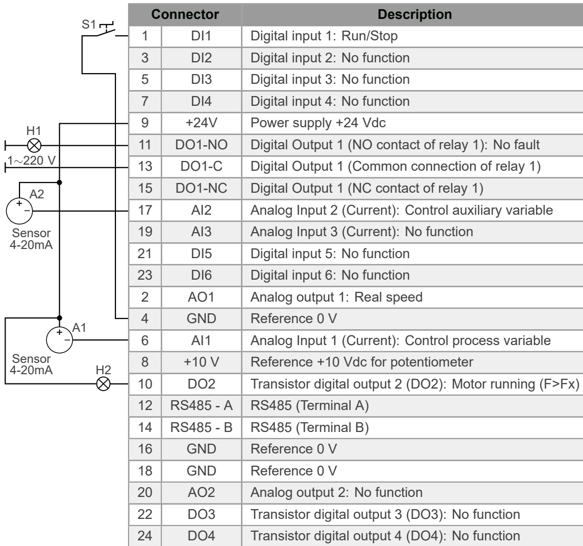
Figure 4.12: Signals on connector of the CFW500-IOAD plug-in module for pump protection via control auxiliary variable
