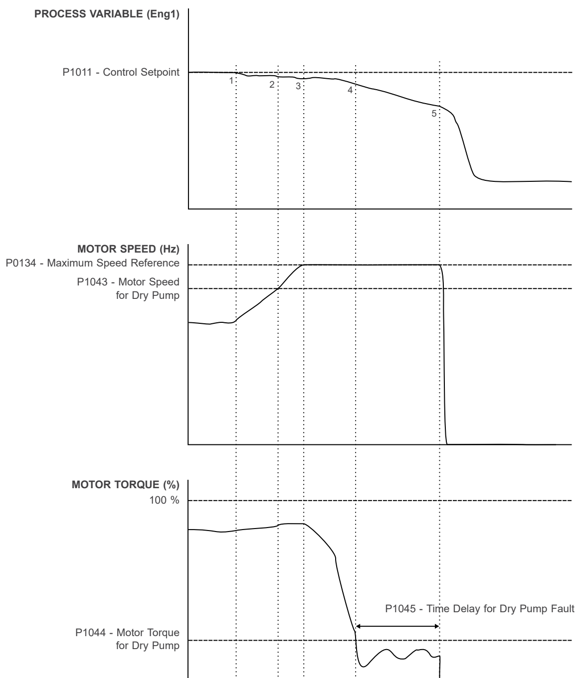
Figure 5.7: Operation of the Pump Genius for dry pump protection
