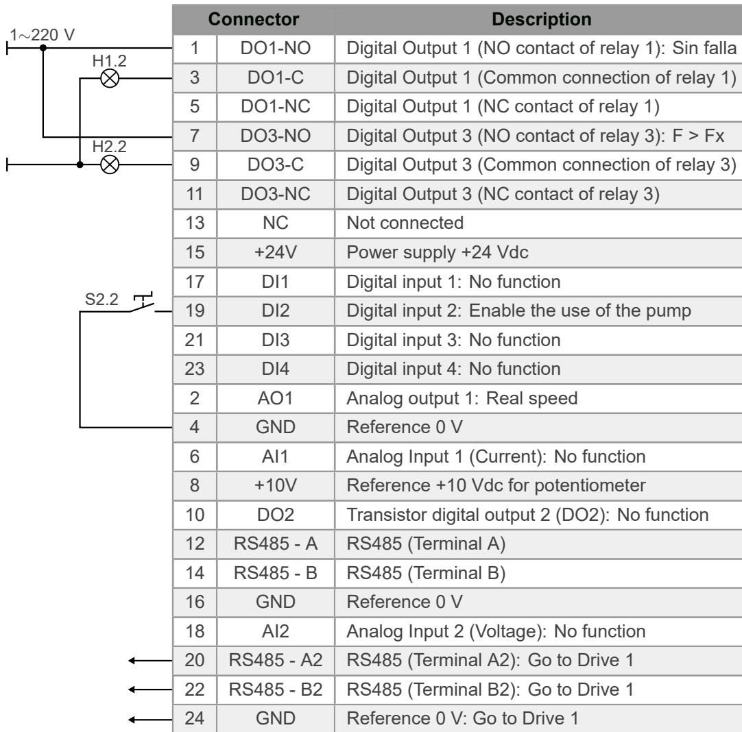
Figure 4.17: Signals on connector of the CFW500-RS485 plug-in module for slave pump (Pump 2)
