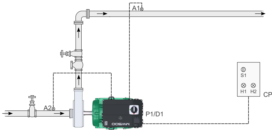
Figure 4.11: Pump Genius Simplex application and pump protection via control auxiliary variable read by analog input
