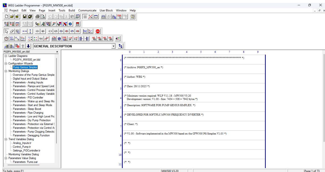
Figure 6.8: Select the configuration wizard for Pump Genius Simplex
