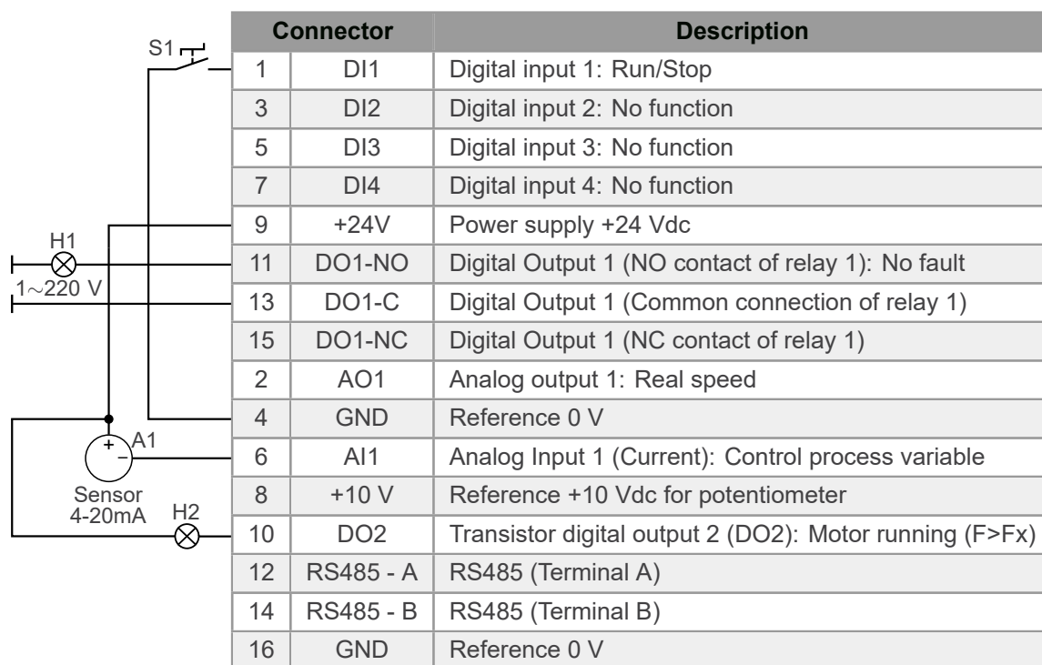
Figure 4.2: Signals on connector of the CFW500-IOS plug-in module for setpoint via HMI
