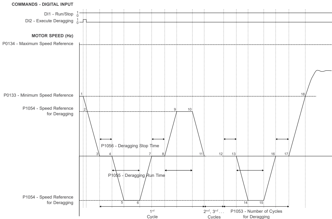
Figure 5.10: Deragging pump operation with command via digital input DI2
