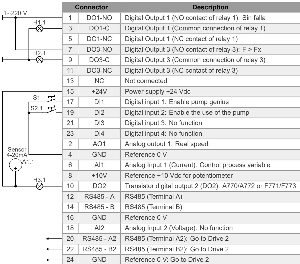
Figure 4.28: Signals on connector of the CFW500-RS485 plug-in module for master/slave pump (Pump 1)
