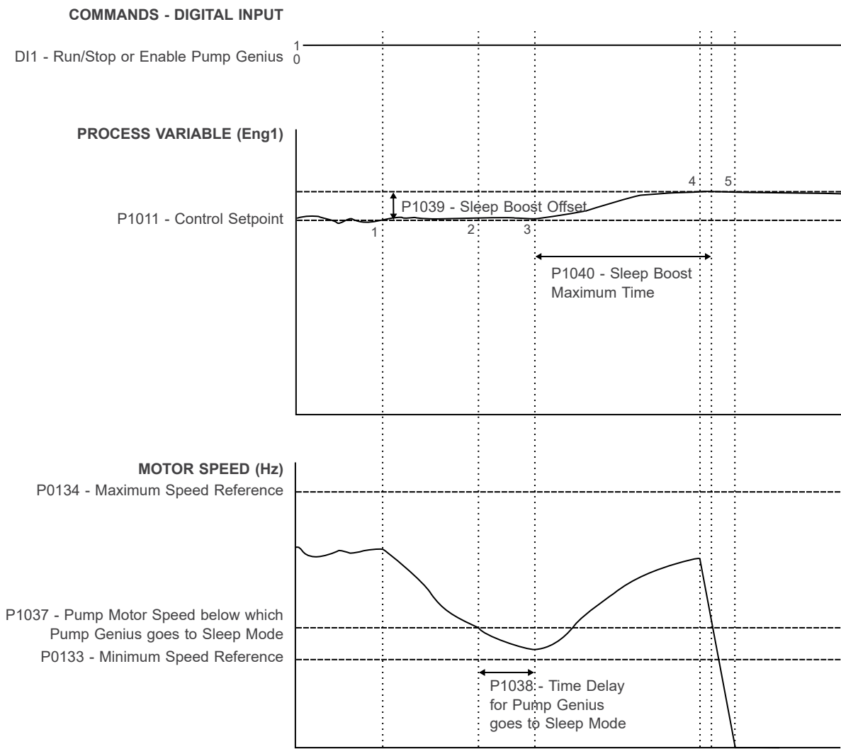
Figure 5.3: Operation of the Pump Genius for sleep mode with sleep boost enabled
