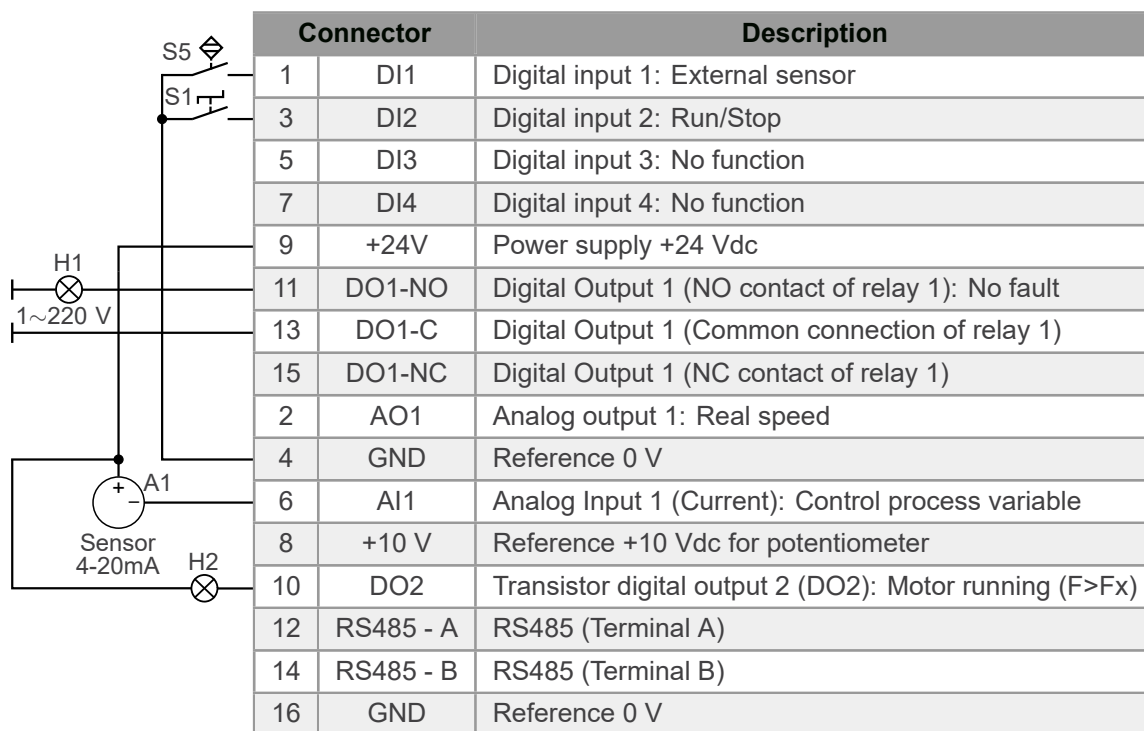
Figure 4.10: Signals on connector of the CFW500-IOS plug-in module for pump protection via external sensor in the digital input DI1
