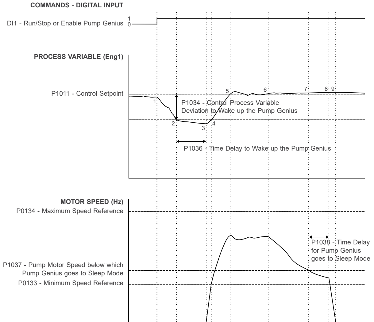
Figure 5.1: Pump Genius operation for Wake up and Sleep mode
