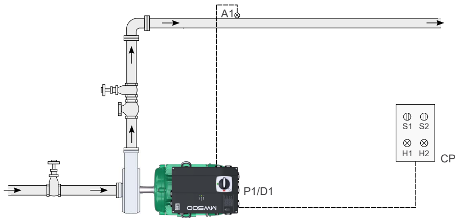
Figure 4.13: Pump Genius Simplex application and deragging function with command via digital input DI2
