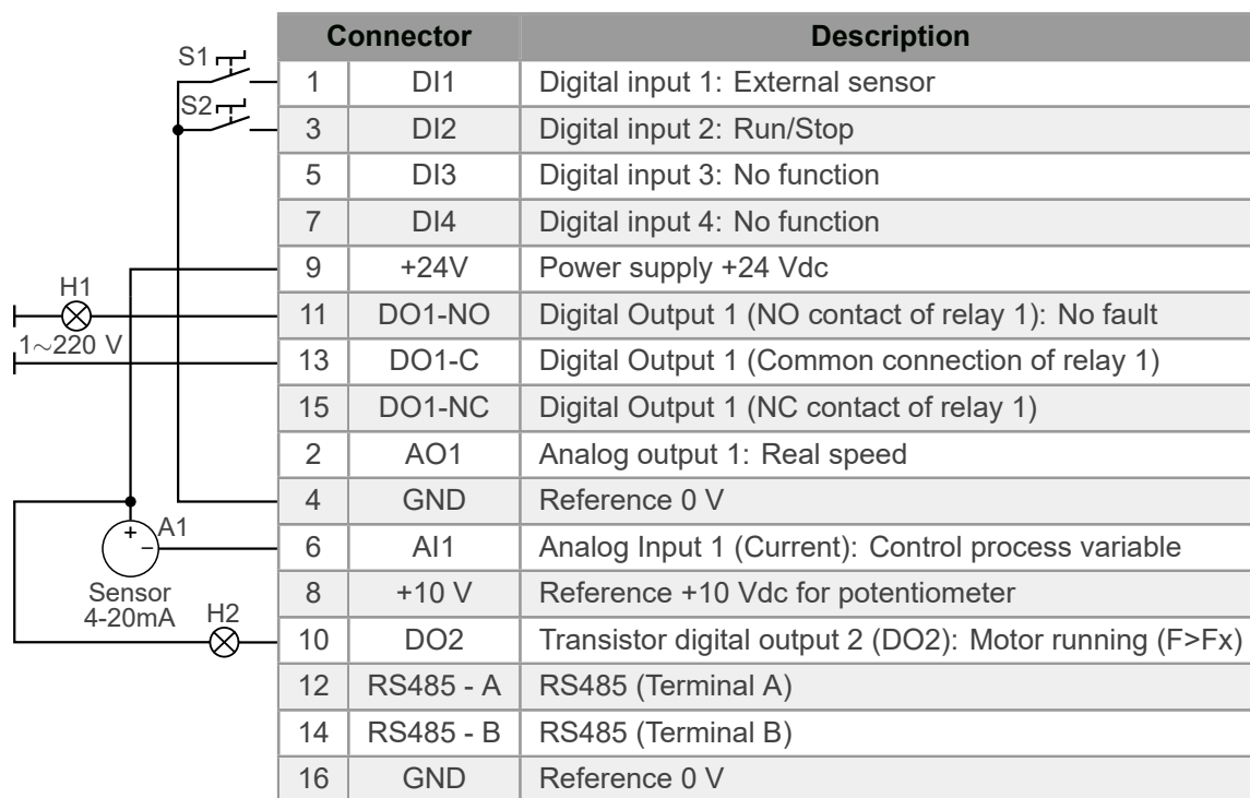
Figure 4.14: Signals on connector of the CFW500-IOS plug-in module for deragging function with command via digital input DI2
