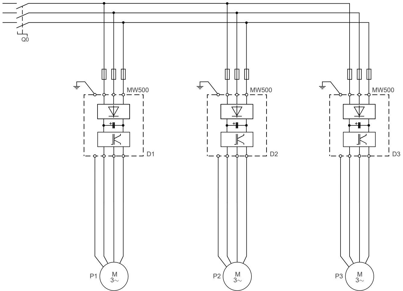
Figure 4.31: Power connections of the Pump Genius Multiplex application with three pumps in parallel
