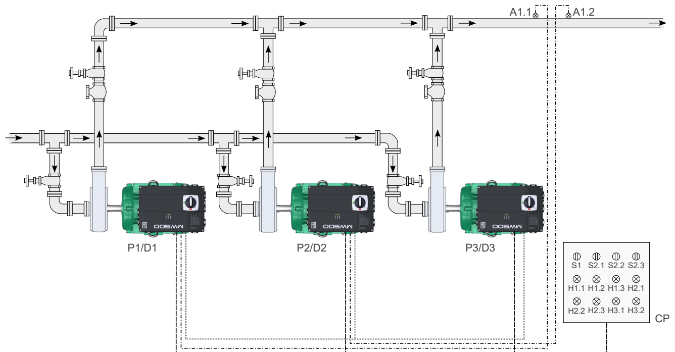
Figure 4.27: Pump Genius Multiplex application with 2 master/slave pumps and one slave pump in parallel and RS485 communication interface
