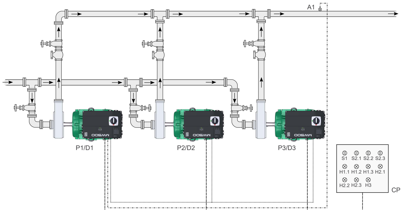
Figure 4.20: Pump Genius Multiplex application with 1 master Pump and two slave pumps in parallel and RS485 communication interface
