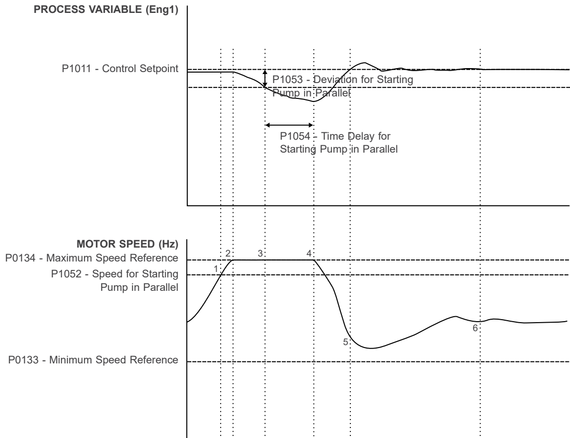
Figure 5.5: Pump Genius Multiplex operation for starting an additional pump in parallel
