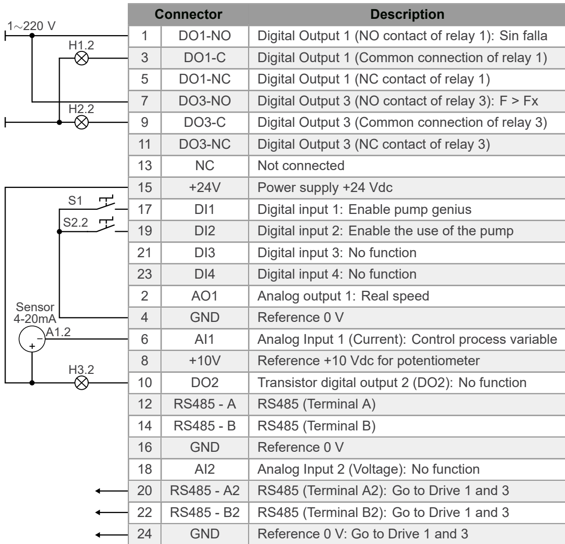
Figure 4.29: Signals on connector of the CFW500-RS485 plug-in module for master/slave pump (Pump 2)
