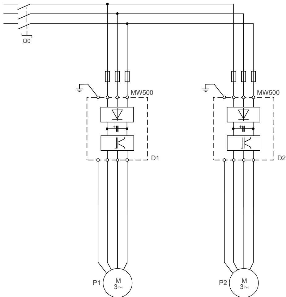
Figure 4.18: Power connections of the Pump Genius Multiplex application with two pumps in parallel
