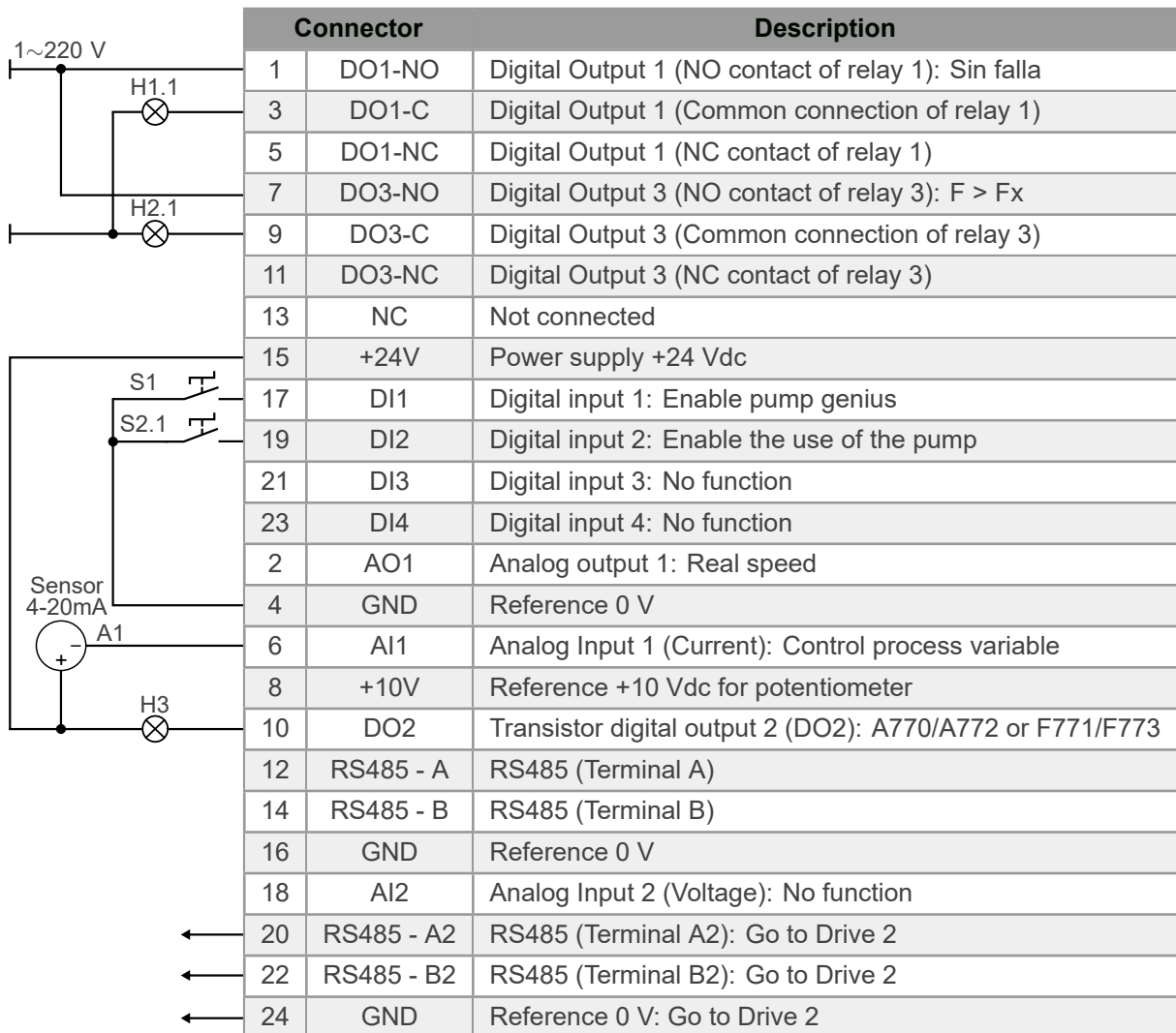
Figure 4.16: Signals on connector of the CFW500-RS485 plug-in module for master/slave pump (Pump 1)
