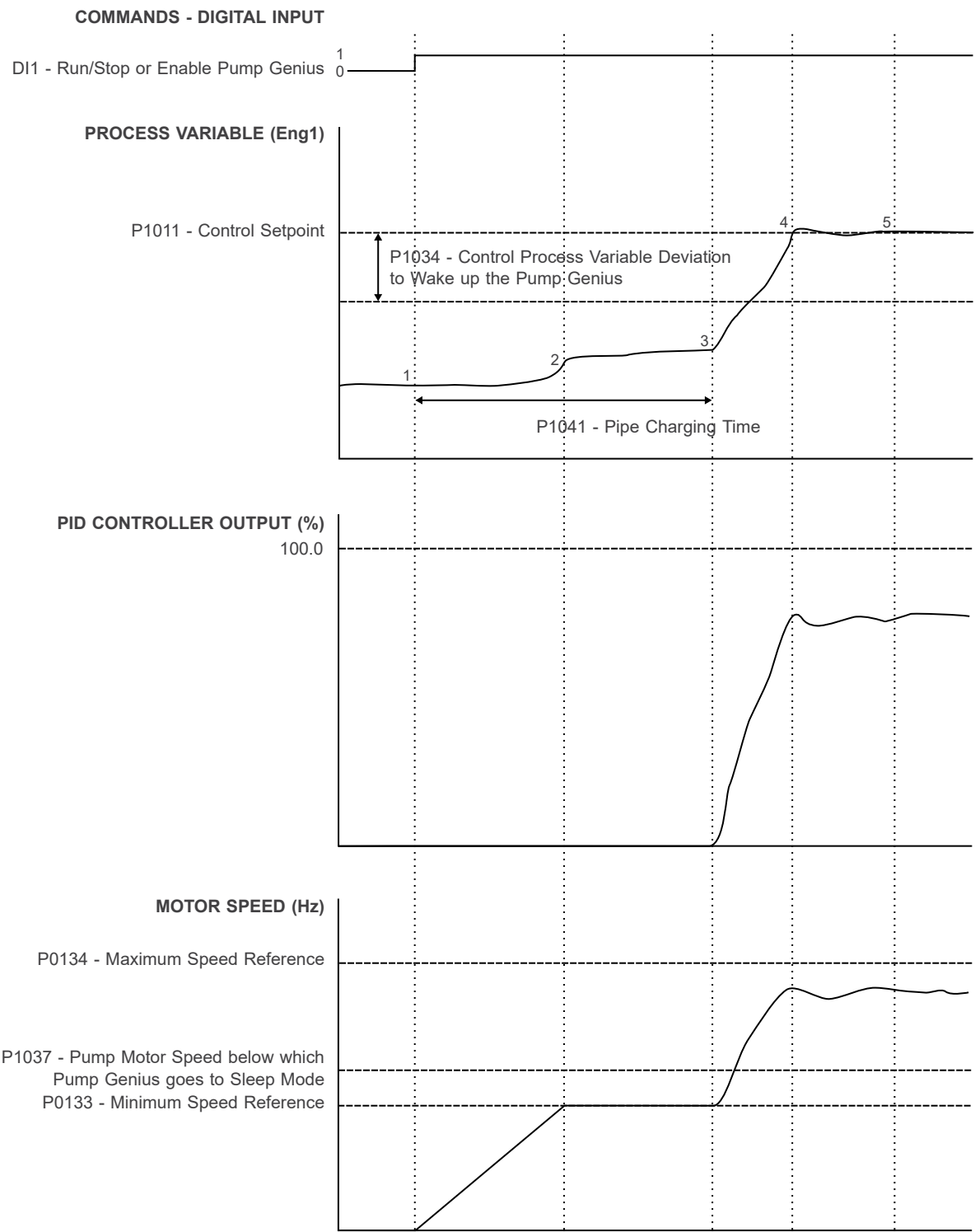
Figure 5.4: Operation of the Pump Genius with pipe charging enabled
