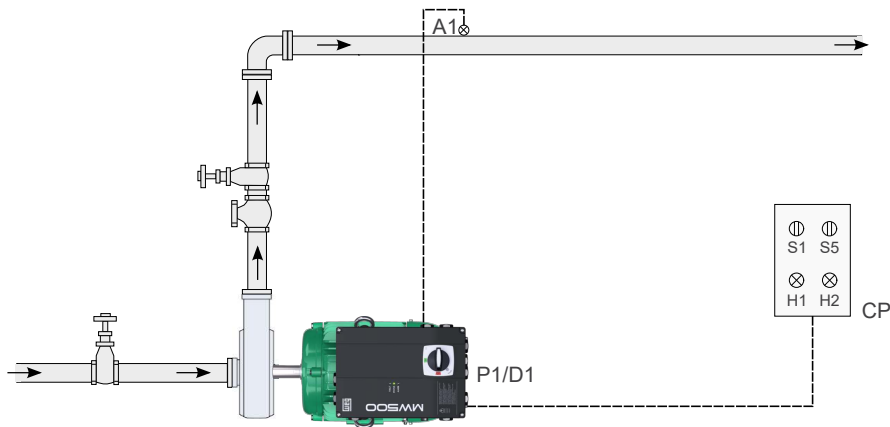
Figure 4.7: Pump Genius Simplex application and selection of PID controller in manual or automatic via digital input DI3
