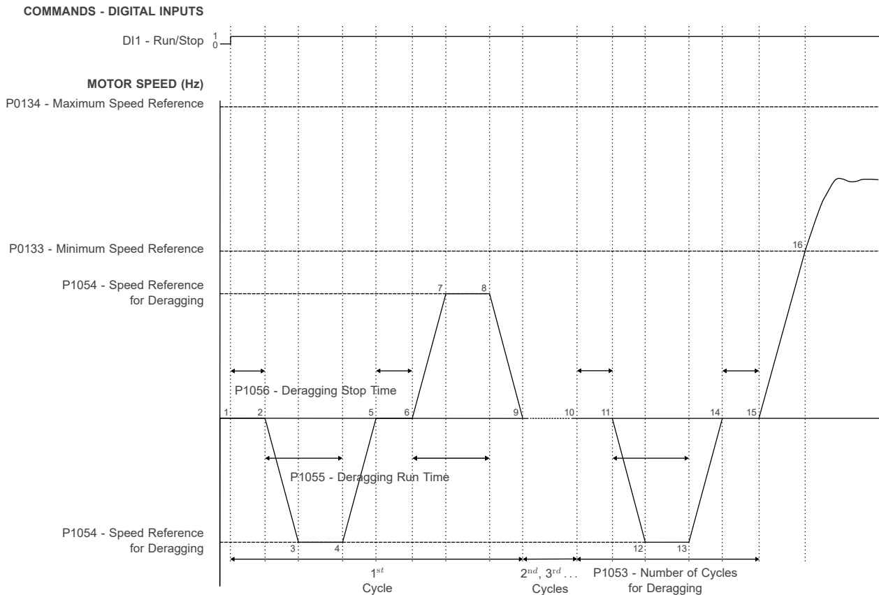
Figure 5.9: Deragging pump operation with command to run the pump
