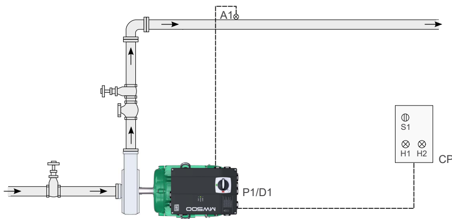
Figure 4.1: Pump Genius Simplex application and control setpoint via HMI
