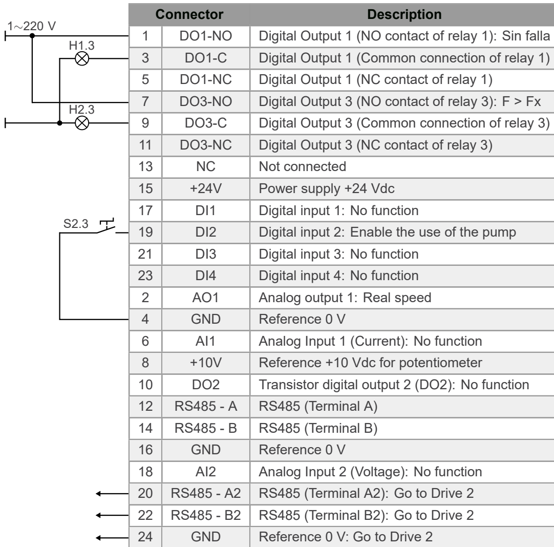
Figure 4.23: Signals on connector of the CFW500-RS485 plug-in module for slave pump (Pump 3)
