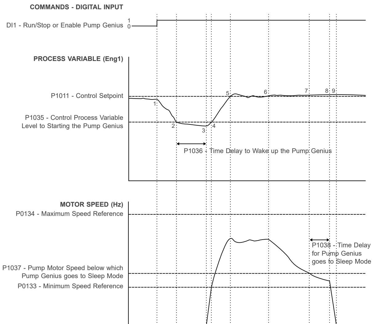
Figure 5.2: Operation of the Pump Genius for start level mode and sleep mode
