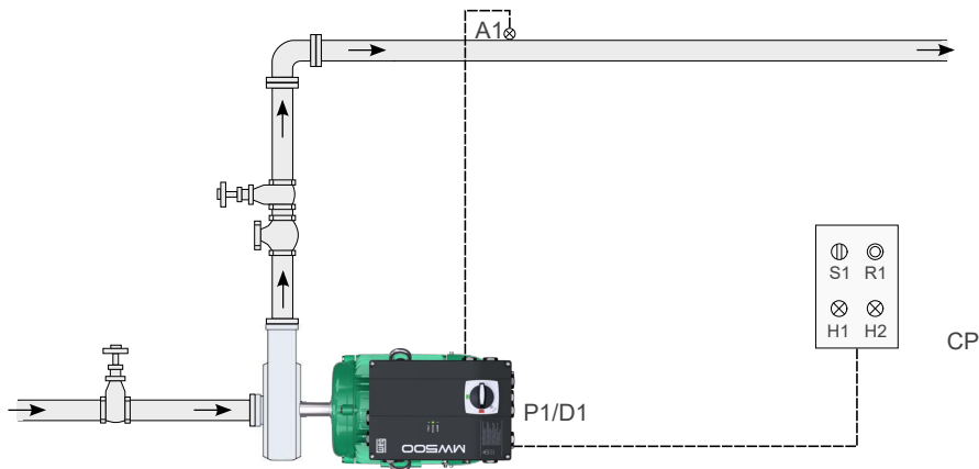
Figure 4.3: Pump Genius Simplex application and control setpoint via analog input
