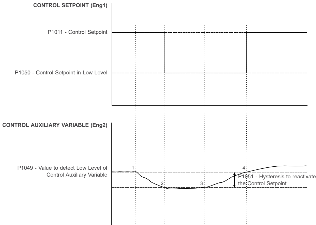
Figure 5.8: Pump Genius operation with pump protection via control auxiliary variable
