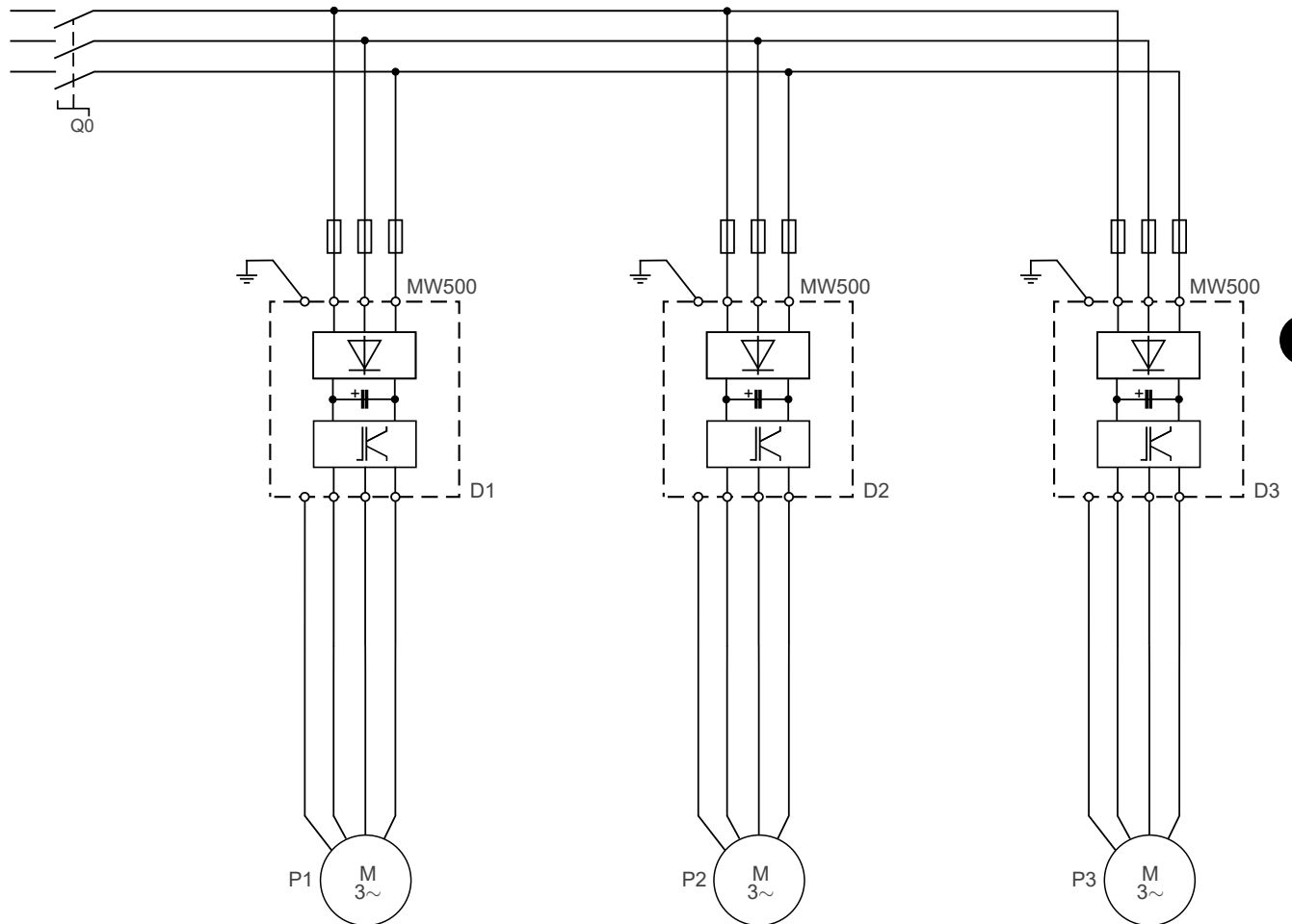
Figure 4.24: Power connections of the Pump Genius Multiplex application with three pumps in parallel
