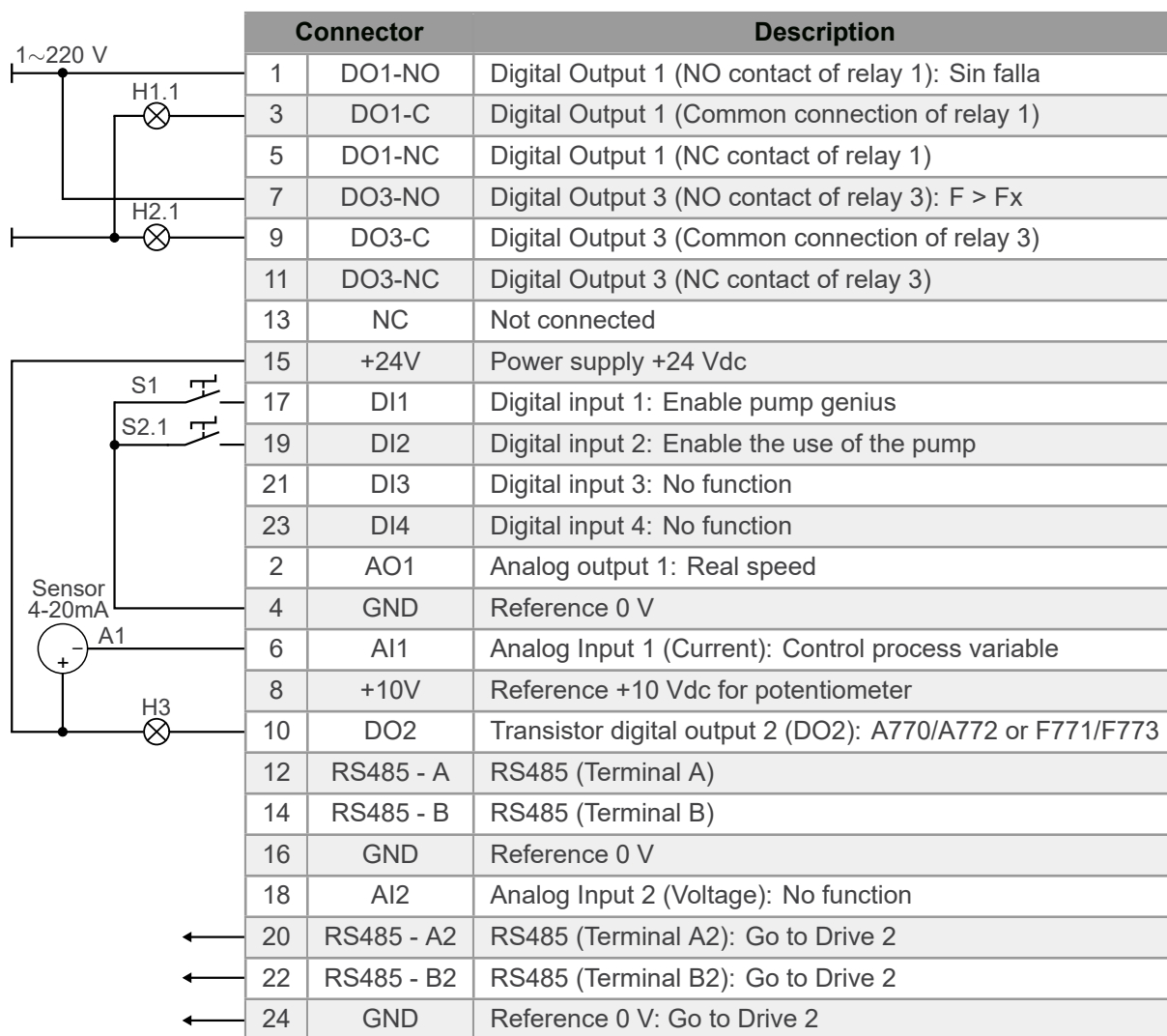
Figure 4.21: Signals on connector of the CFW500-RS485 plug-in module for master/slave pump (Pump 1)
