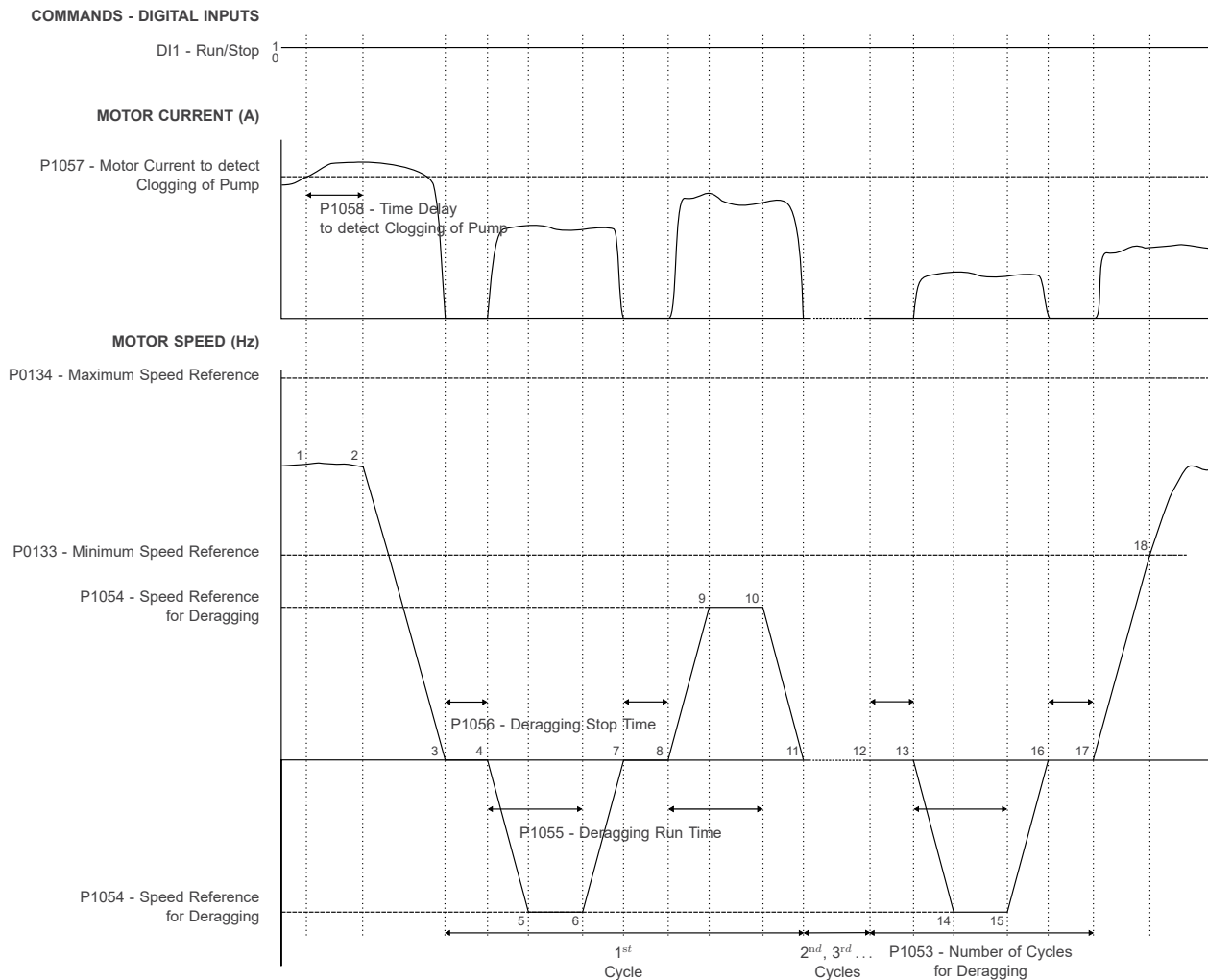
Figure 5.11: Deragging pump operation when a clogging of pump is detected
