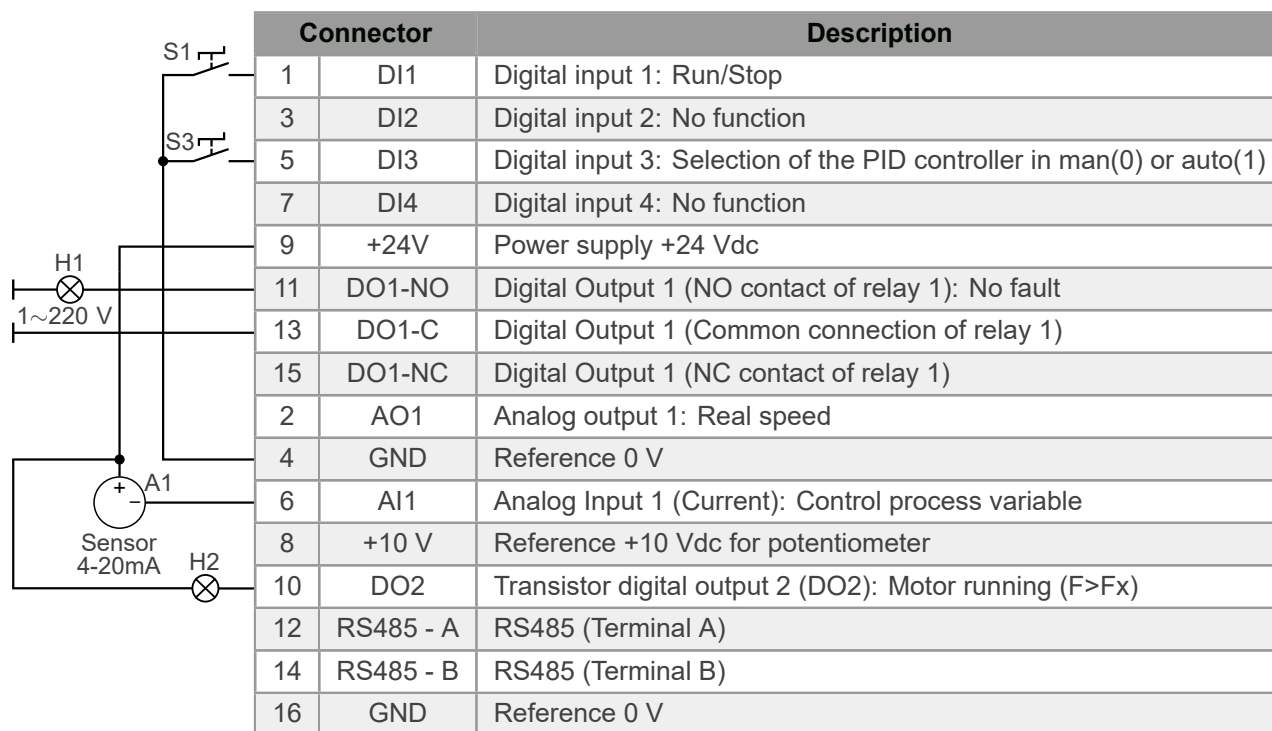
Figure 4.8: Signals on connector of the CFW500-IOS plug-in module for setpoint for Selection of the PID controller in Manual / Automatic via DI3
