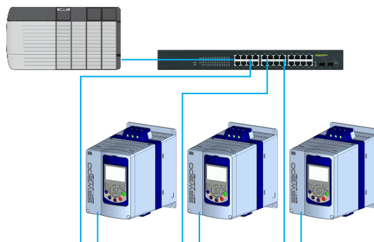
Figure 3.1: Star topology
