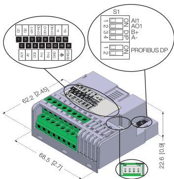
Figure A.3: CPDP2 dimensions in mm [in], DIP-switches location and MCard connector
