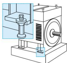
Figura 4.10: Chumbadores
