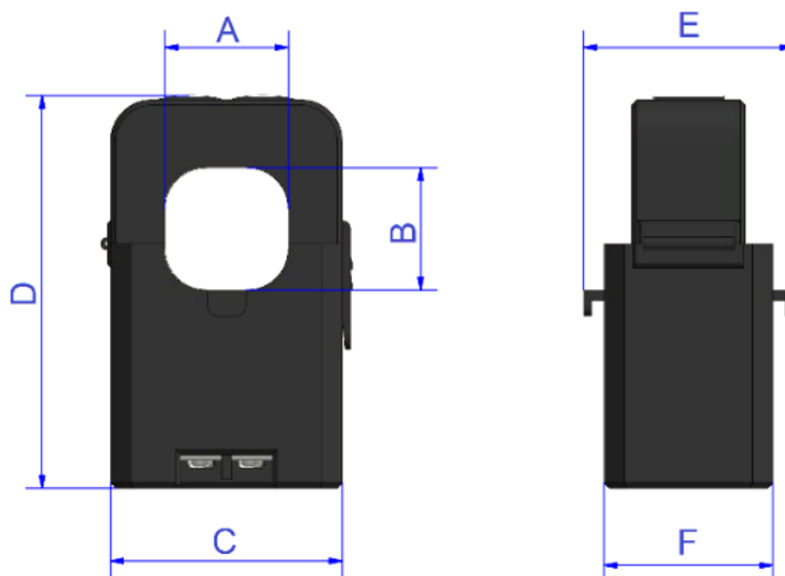
Figura 3 – Sensor Split Core
