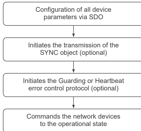
Figure 7.7: Initialization process flowchart
