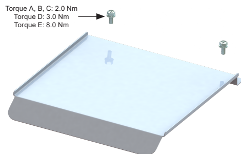
Figure 1.2: Exploded KIP21 A-B-C-D-E kit mounting
