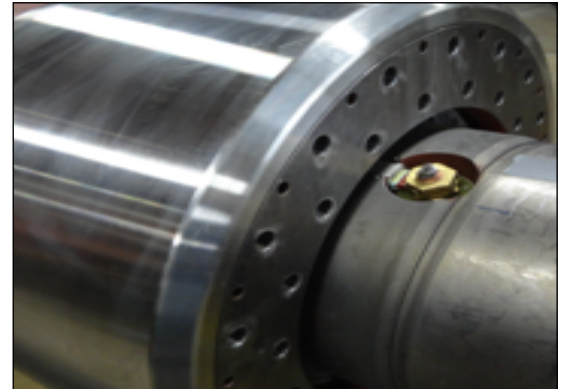
Rotor Coils with Ventilation Slots
