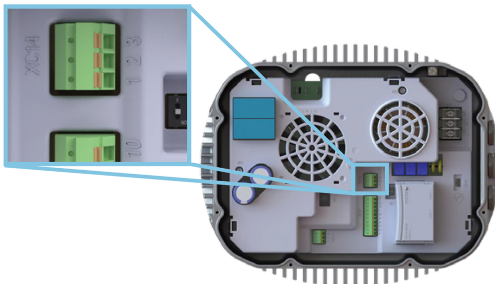
Figure 6.3: XC14 Terminal Block
