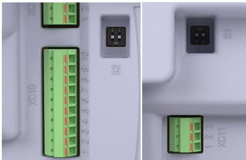
Figure 5.5: Left: XC10 terminal block (Main input and outputs of the product)) and S2 keys (RS 485 resistors), Right: XC11 terminal block (Digital output 1, relay contacts) and S1 keys (forced serial communication)
