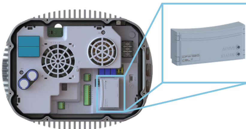
Figure 6.6: Connect a Bluetooth module to the XC3 connector
