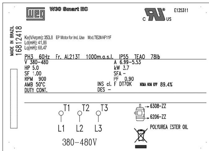
Figure 4.1: Nameplate
