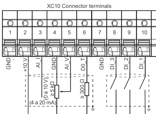
Figure 6.2: Drive terminal blocks and ports
