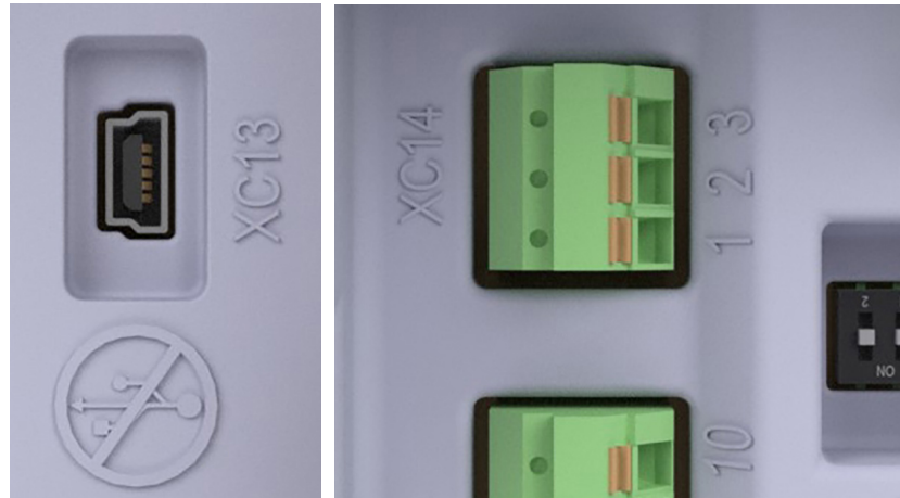
Figure 5.6: Left: XC13 terminal block (HMI input), Right: XC14 terminal block (Modbus RTU input)
