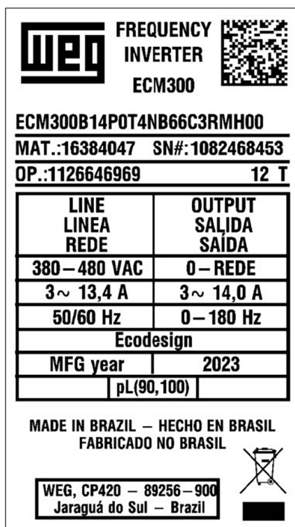
Figure 4.2: Drive label
