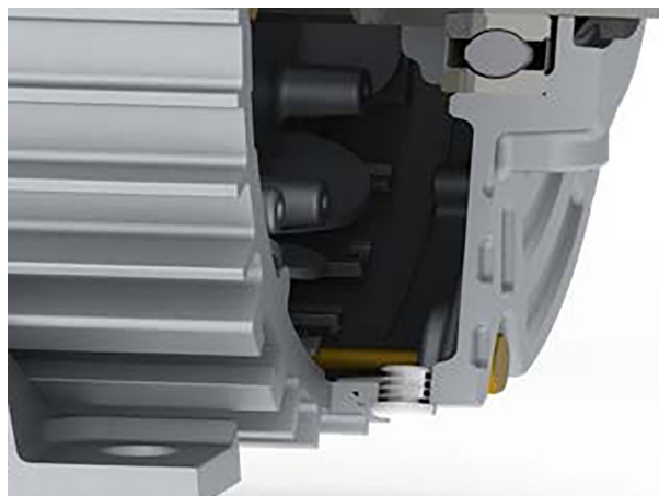
Figure 5.3: Drain sectional view
