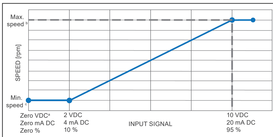
Figure 6.1: Control input reference
