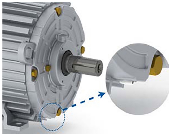
Figure 5.2: Drain Position
