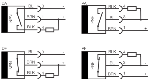
Figure 1: Electric diagram
