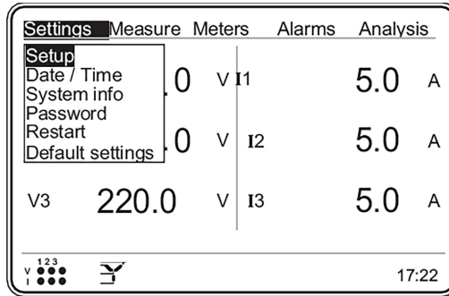
Figure 3.11: Settings menu
