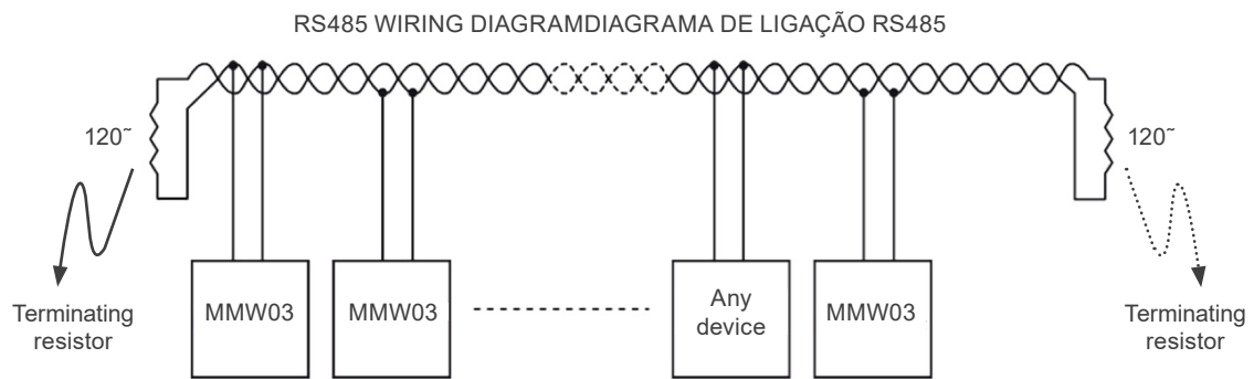
Figure 4.1: RS485 wiring diagram
