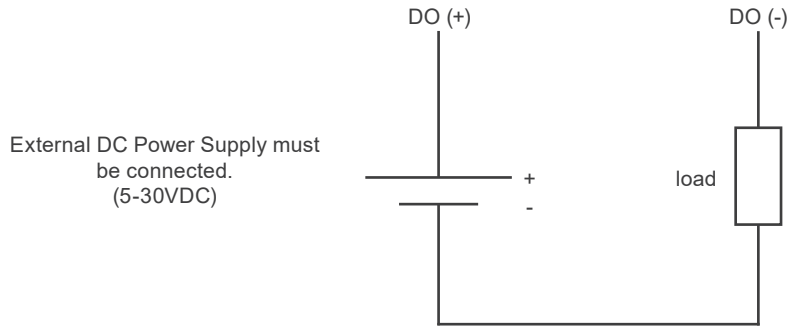
Figure 2.12: Digital output connection diagram
