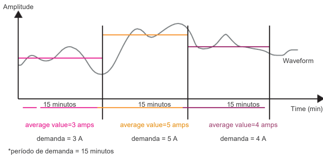
Figure 3.63: Demand example
