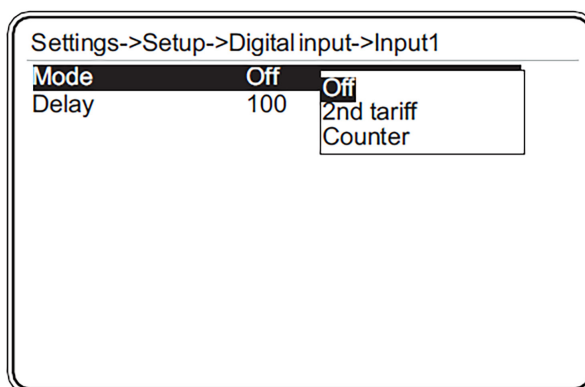
Figure 3.30: Mode selection
