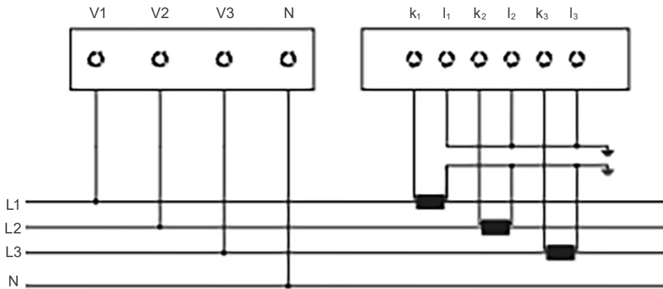
Figure 2.7: Star connection - Direct measurement of voltage and current with 3 CTs
