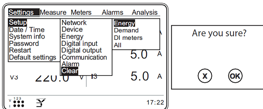
Figure 3.50: Clear Menu
