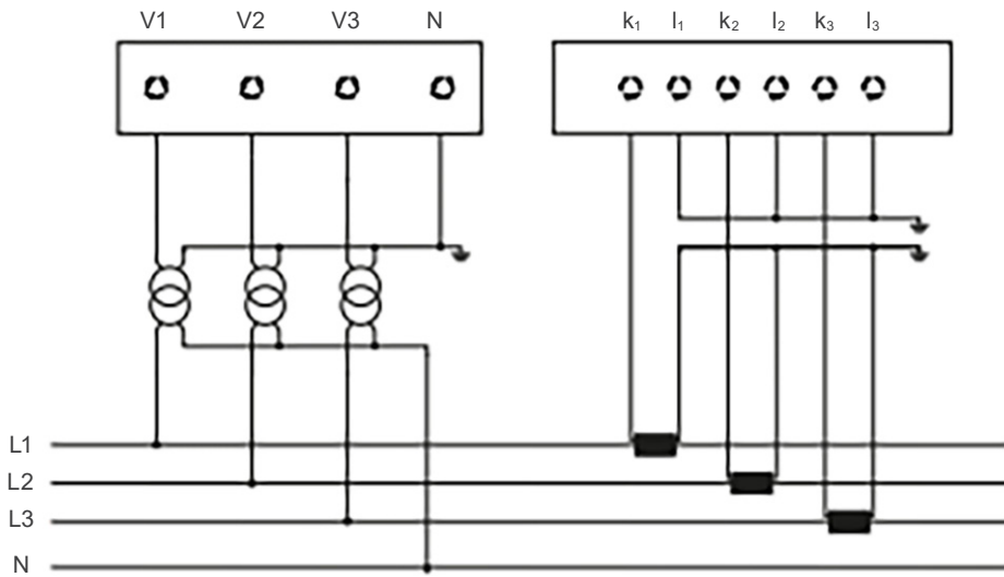
Figure 2.6: Star connection - Measurement with 3 PTs and 3 CTs
