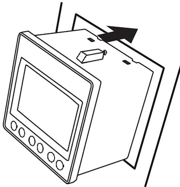
Figure 2.1: Mounting MMW03-M22CHb into the panel
