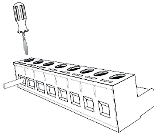
Figure 2.5: Fixing the cable to the terminal block
