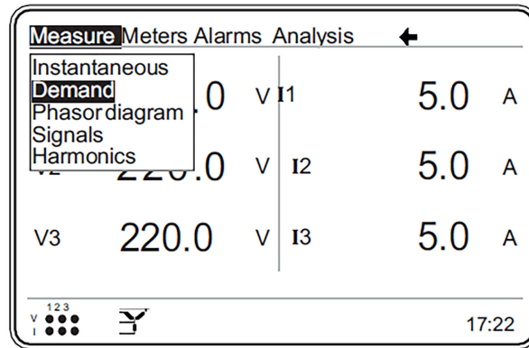
Figure 3.62: Demand menu
