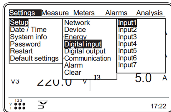
Figure 3.29: Digital input menu (With IO option)
