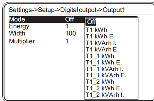
Figure 3.35: Output1 menu
