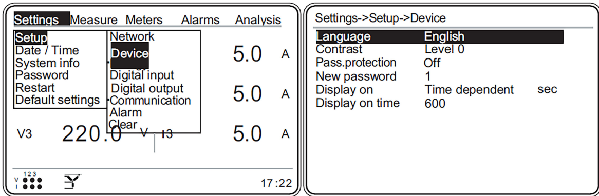
Figure 3.19: Device menu
