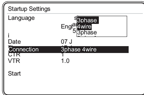
Figure 3.8: Connection types
