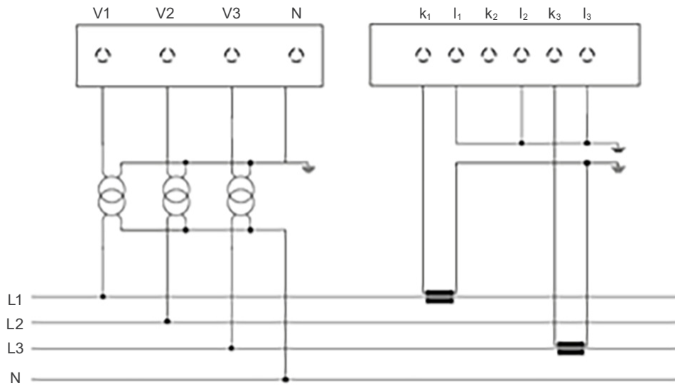
Figure 2.8: Star connection - Measurement with 3 PTs and 2 CTs
