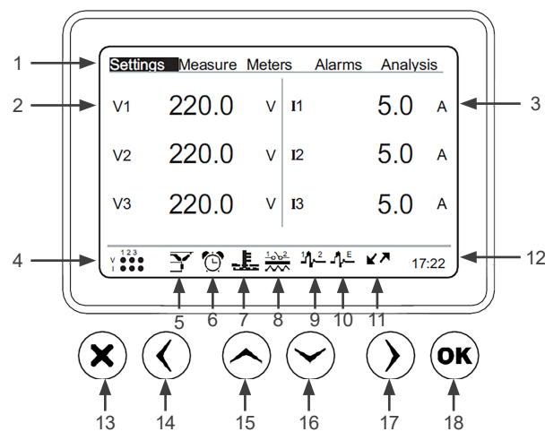
Figure 1.1: MMW03-M22CHB display
