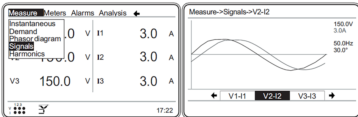
Figure 3.68: Signals menu
