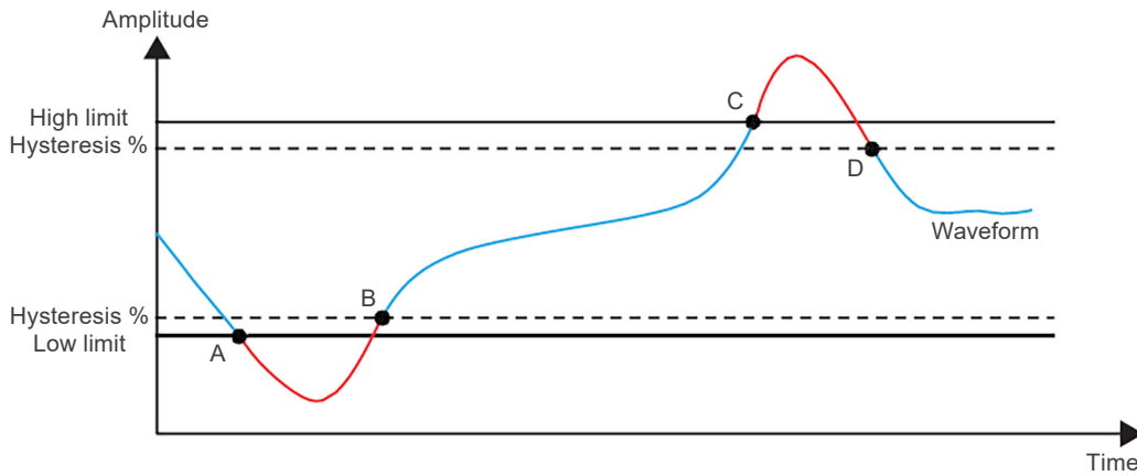
Figure 3.44: Alarm example
