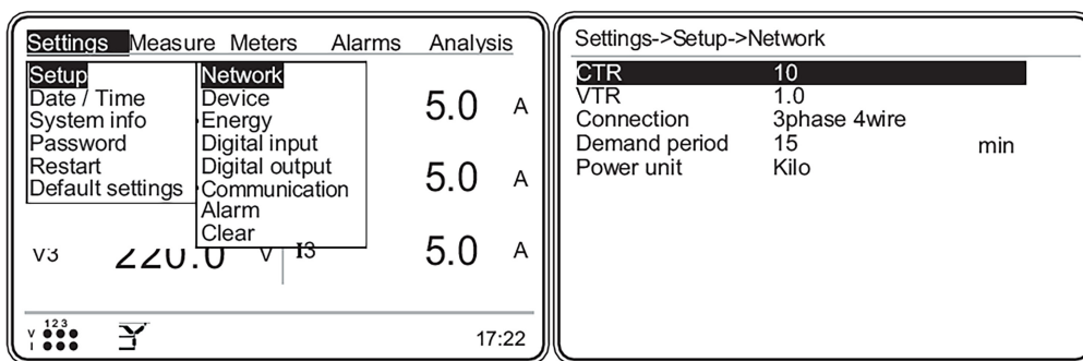
Figure 3.13: Network menu
