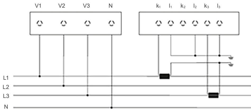
Figure 2.9: Star connection - Direct measurement of voltage and current with 2 CTs (ARON)
