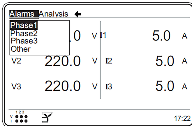
Figure 3.82: Alarms menu
