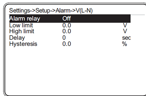
Figure 3.40: V(L-N) menu
