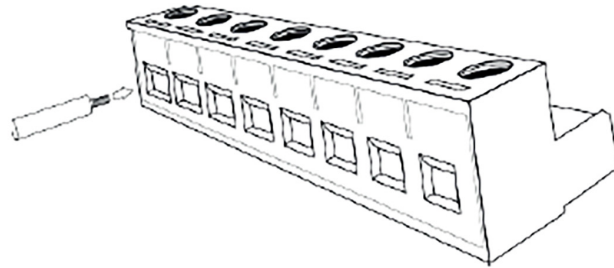
Figure 2.4: Inserting cable into the terminal block
