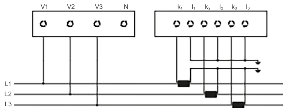
Figure 2.10: Delta connection - Direct measurement of voltage and current with 3 CTs
