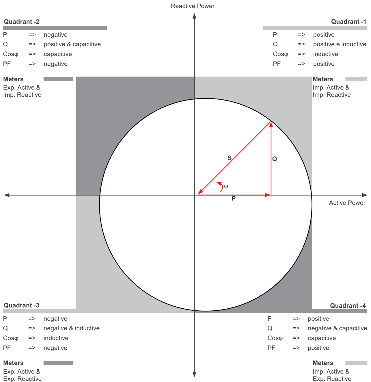
Figure 1.2: Four-quadrant representation
