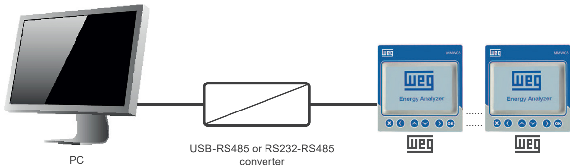
Figure 4.2: Connection of MMW03-M22CHB to a PC
