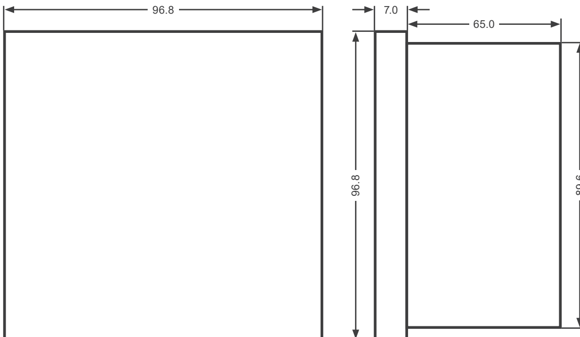
Figure 2.13: Dimensions
