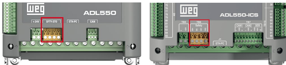
Figure 6 - STO connector
