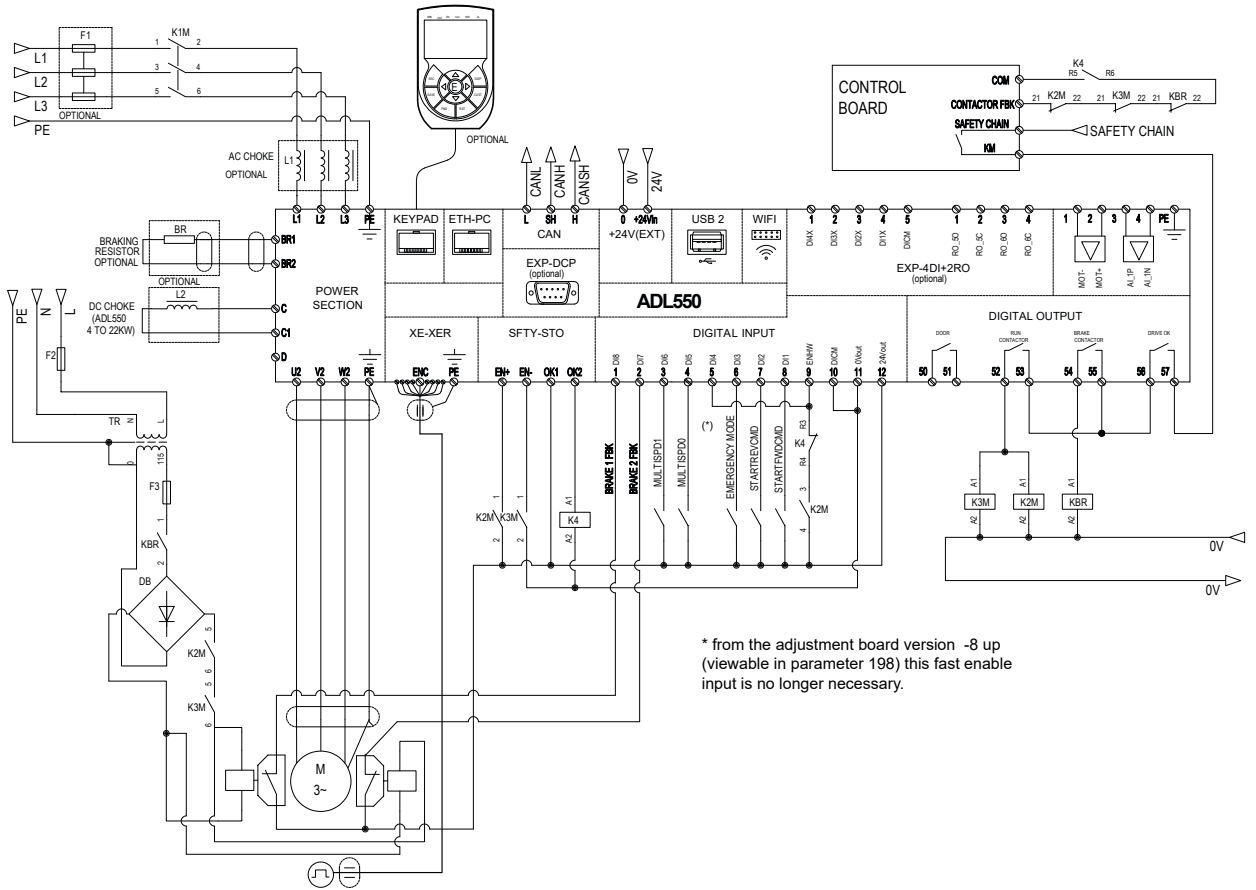
Figure 11 - ADL550 contactor – less application design case
