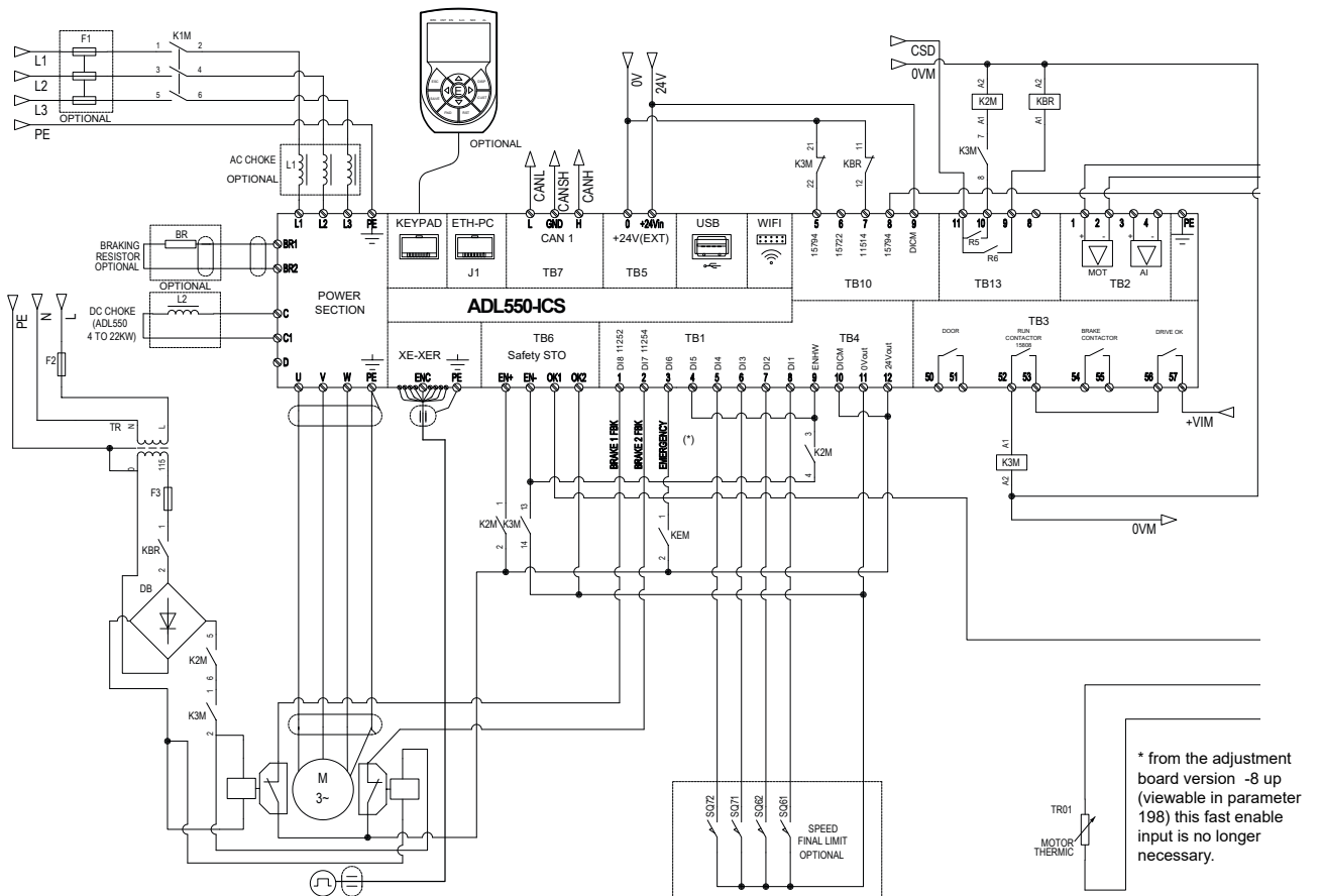
Figure 12 - ADL550-ICS contactor – less application design case
