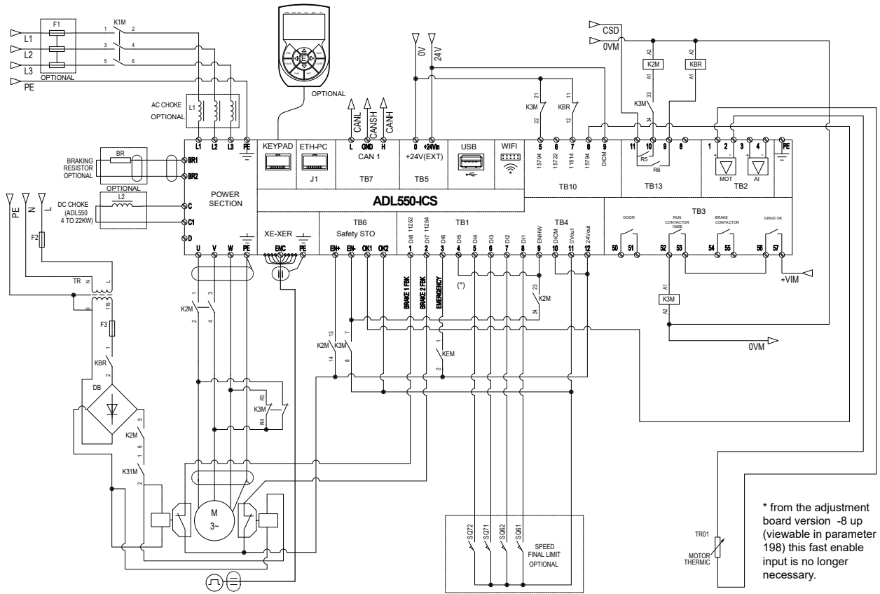
Figure 10 - ADL550-ICS Specific Reference design using a single contactor (onto the AC motor)
