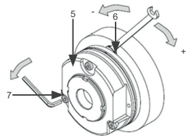
Figure 5.3: Air gap adjustment of the sizes 6 to 25
