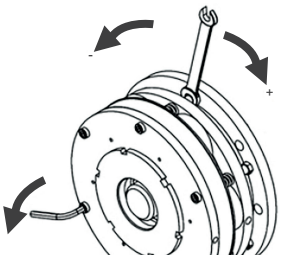
Figure 5.6: Air gap adjustment of the brake sizes 25 and 31
