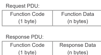
Figure 2.1: Modbus transaction
