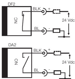
Figure 1: Electric diagram
