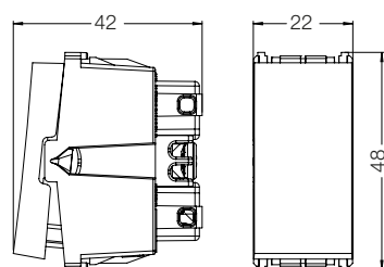
Interruptor simples
