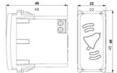
Campainha cigarra
