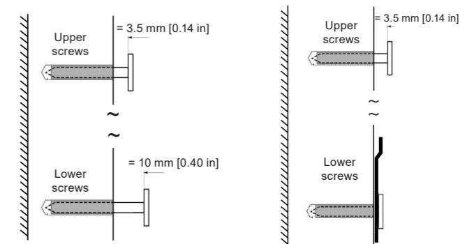
(a) Mounting without the metal bracket (b) Mounting with the metal bracket
