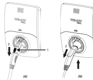
Figure 5.4: (a) and (b) Procedure for removing the plug from the socket on charging stations with cables type 1 and NACS
