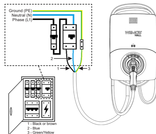
(a) with single-phase circuit breaker and RCD
