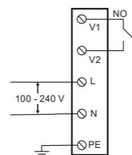
Figure 5.2: Internal electrical connection
