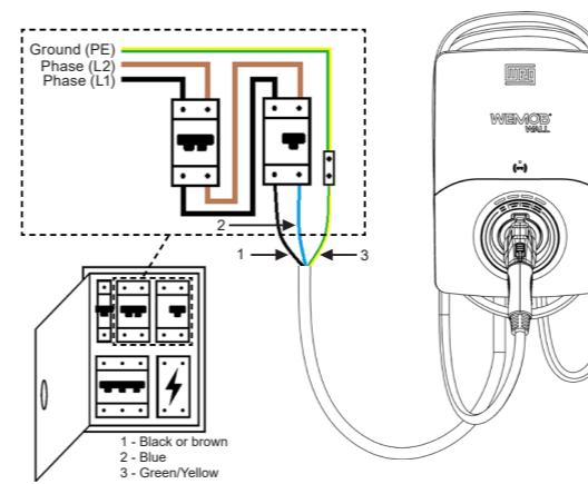
(b) with two-phase circuit breaker and RCD
