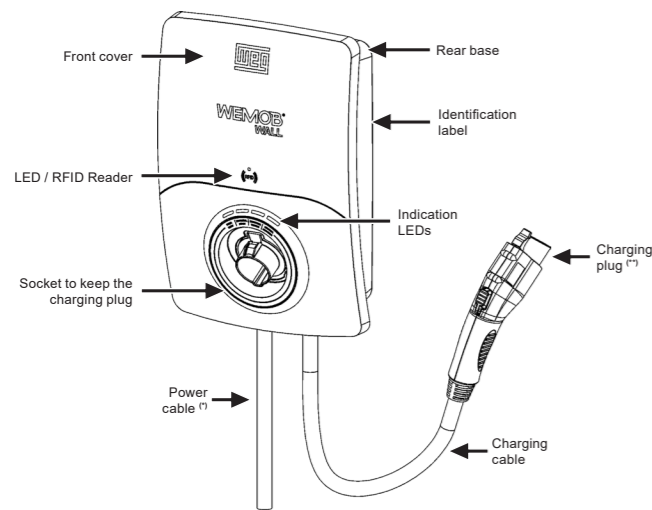
Figure 2.1: WEMOB-WALL overview
