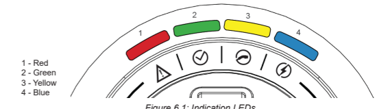
Figure 6.1: Indication LEDs
