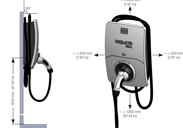
Figure 4.1: Mounting position and spacing of the WEMOB-WALL
