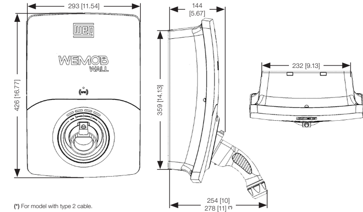
Figure 7.1: Dimensions of the WEMOB-WALL charging station in mm [in]
