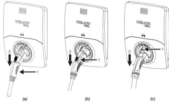
Figure 5.4: (a), (b) and (c) Procedure for removing the plug from the socket on charging stations with cables type 1, GB/T and type 2
