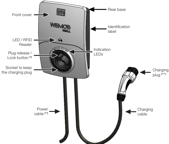
Figure 2.1: WEMOB-WALL overview
