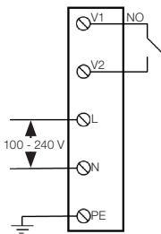
Figure 5.2: Internal electrical connection
