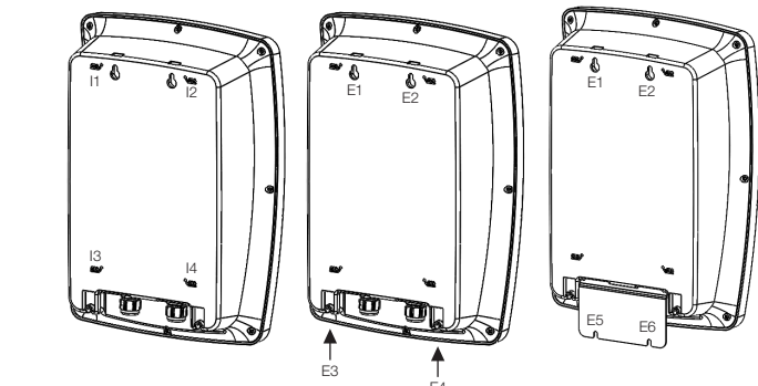
Figure 4.2: WEMOB-WALL mounting methods
