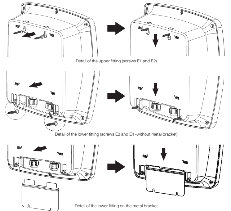
Detail of the lower fitting on the metal bracket
