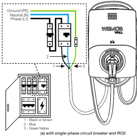
(a) with single-phase circuit breaker and RCD
