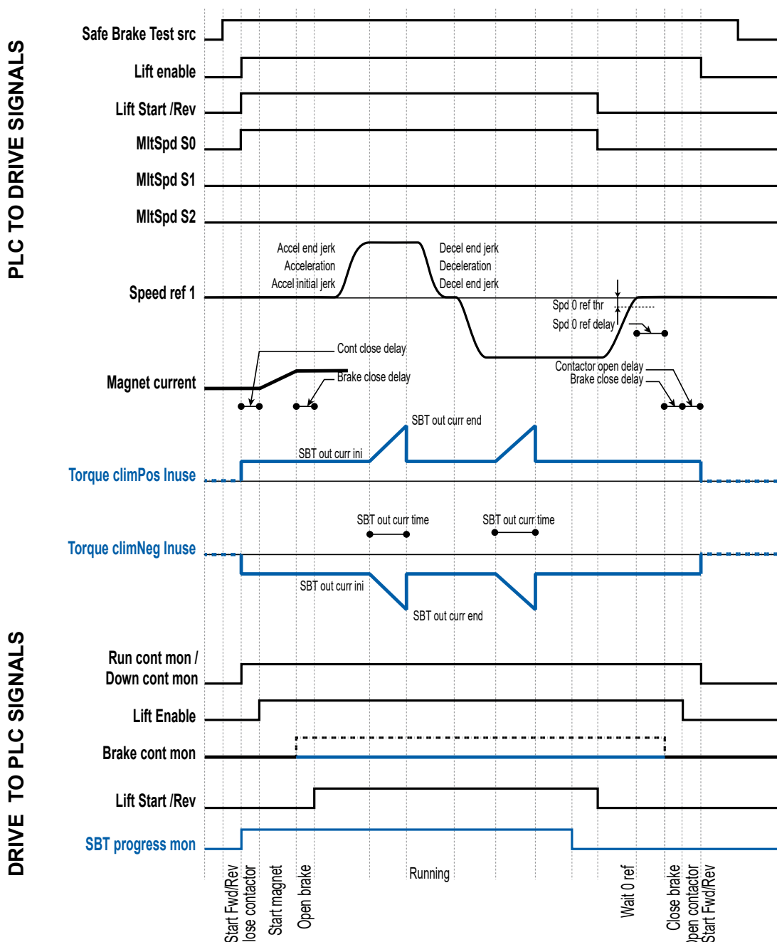
Safe Brake Test command sequence
