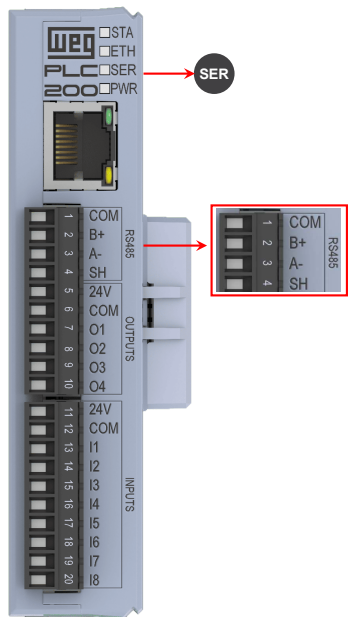
Figure 2.1: Connector and indications for PLC200
