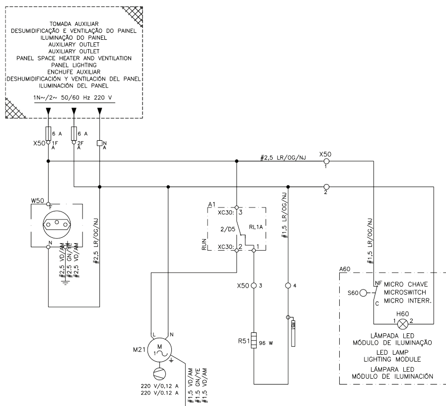
Figure 4.12: Auxiliary circuit electrical detail
