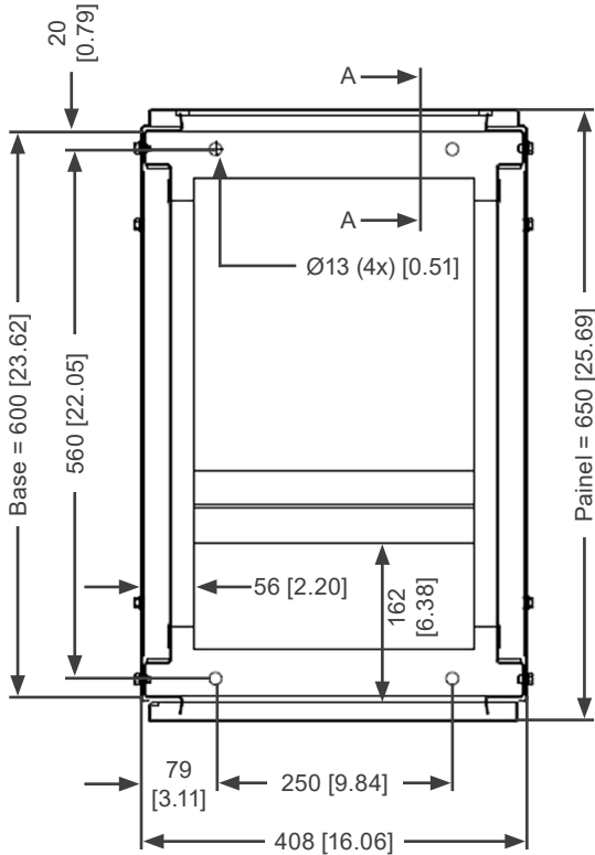
Figure 4.3: Fixing details of AFW900C frame E
