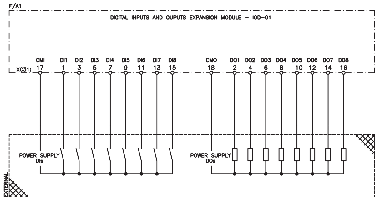
Figure 2.9: IOD-01 electrical connection
