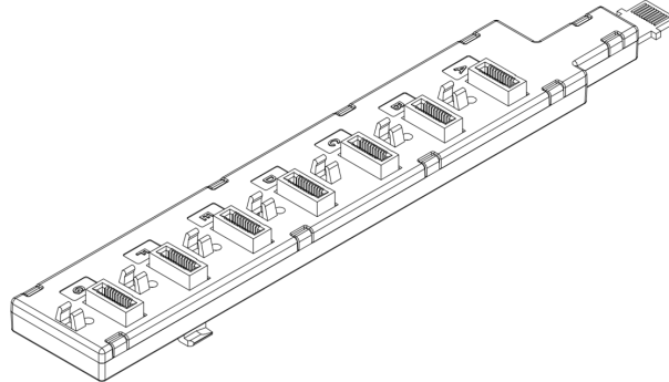
Figure 2.12: 7 Slots Module
