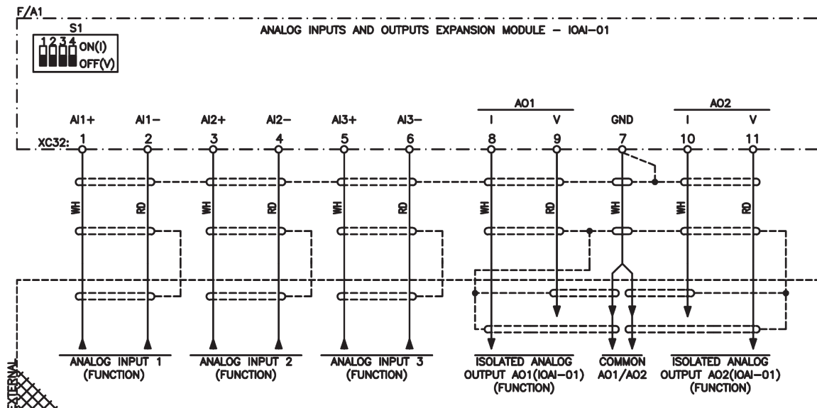
Figure 2.5: IOAI-01 electrical connection
