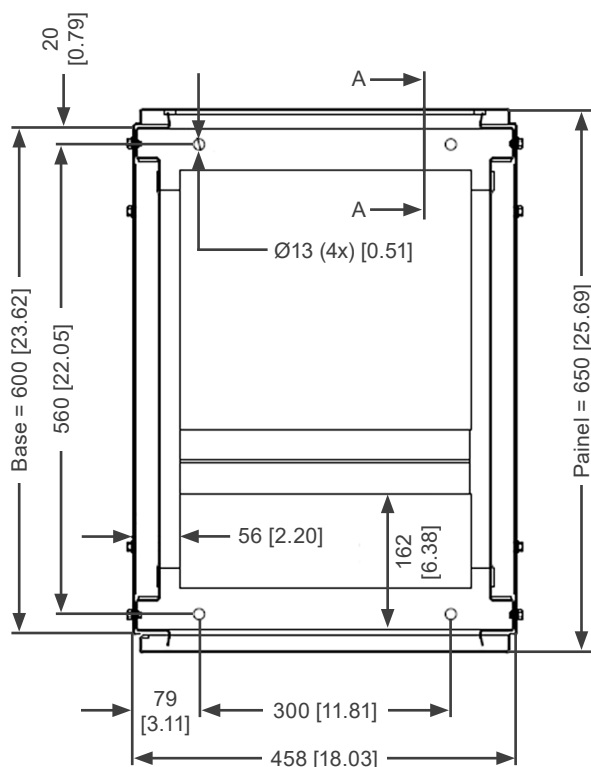
Figure 4.4: Fixing details of AFW900C frame F
