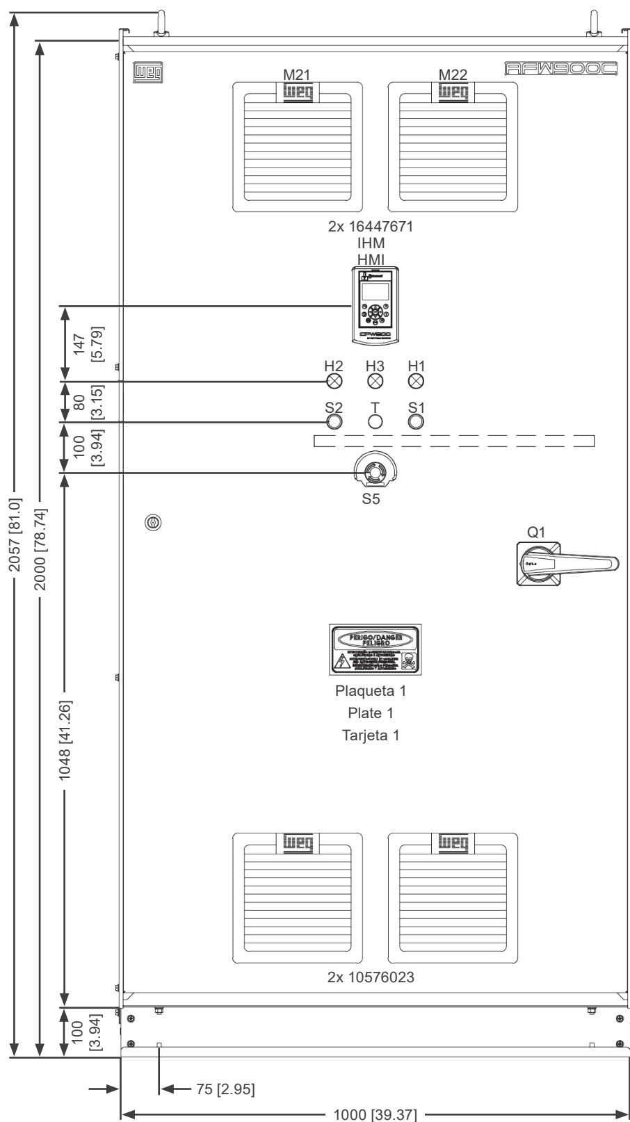
Figure 4.11: Mechanical details of frame H
