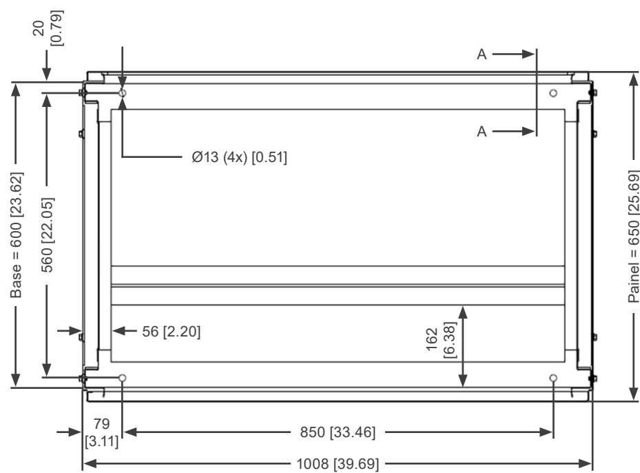
Figure 4.6: Fixing details of AFW900C frame H
