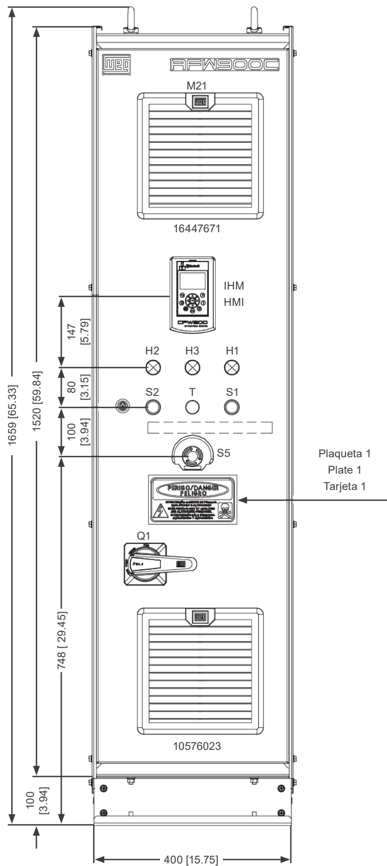
Figure 4.8: Mechanical details of frame E
