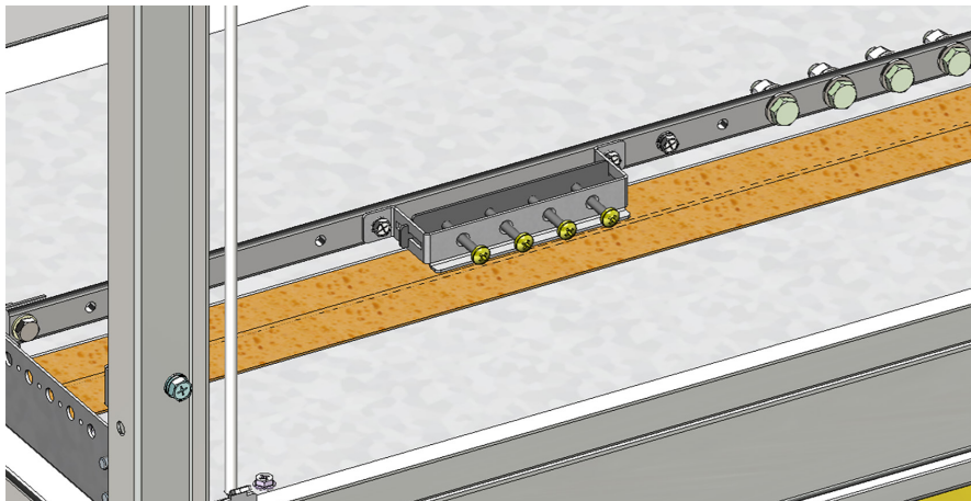
Figure 4.13: Mechanical detail for shielded cable grounding
