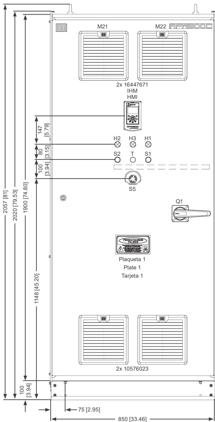
Figure 4.10: Mechanical details of frame G
