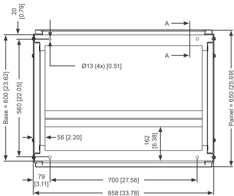
Figure 4.5: Fixing details of AFW900C frame G
