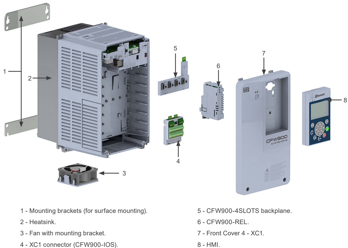
Figure 2.13: Parts of the CFW900 frame A
