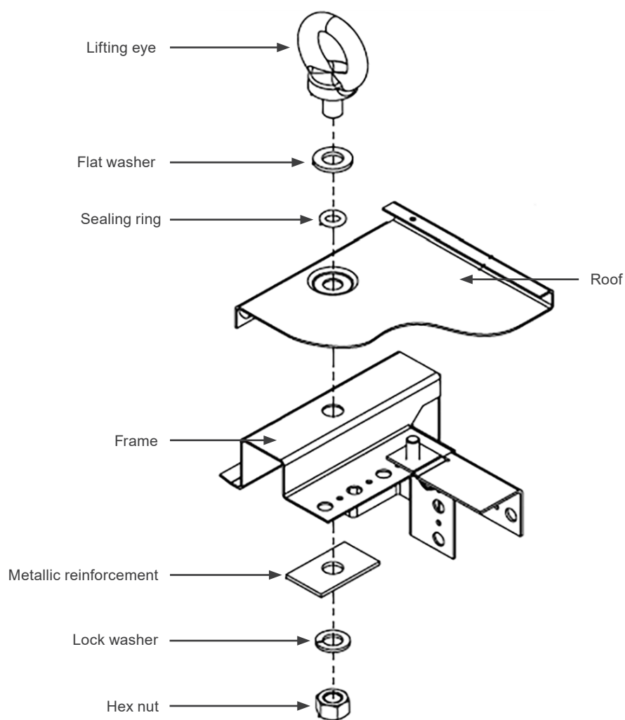
Figure 1.12: Exploded detail lifting eyes
