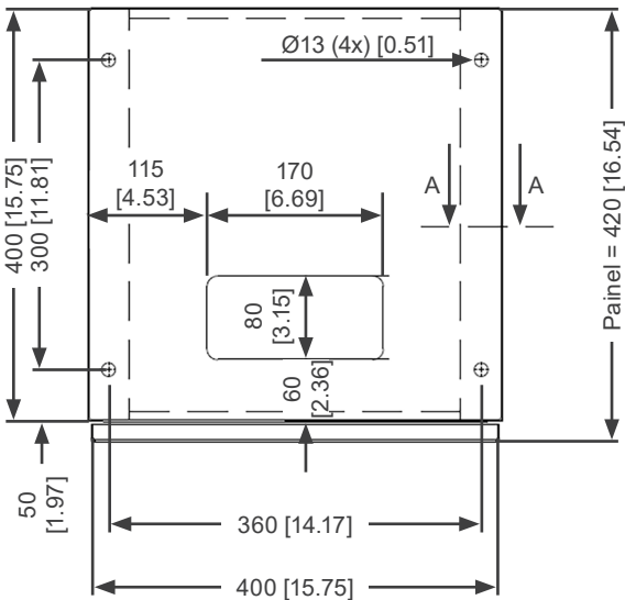
Figure 4.2: Fixing details of AFW900C frames C and D
