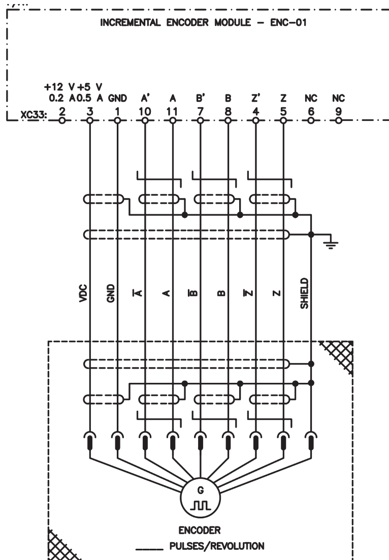
Figure 2.11: ENC-01 electrical connection
