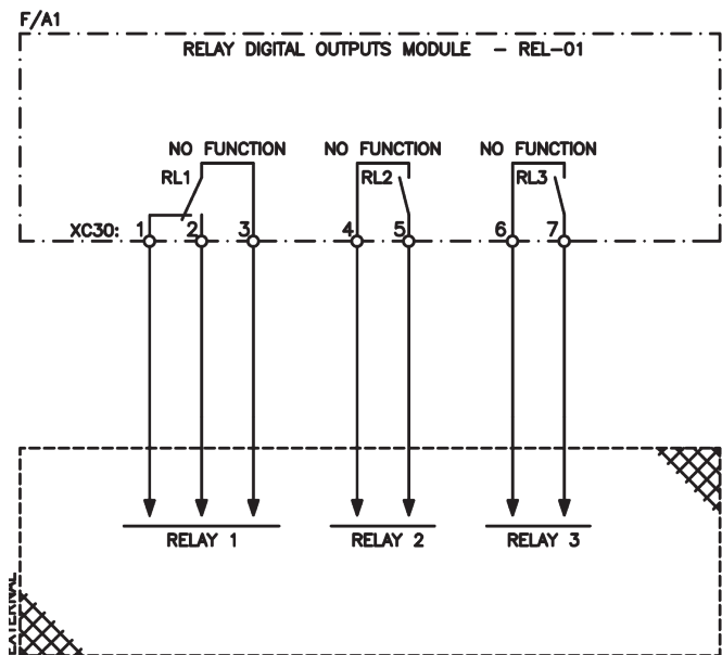
Figure 2.3: REL-01 electrical connection
