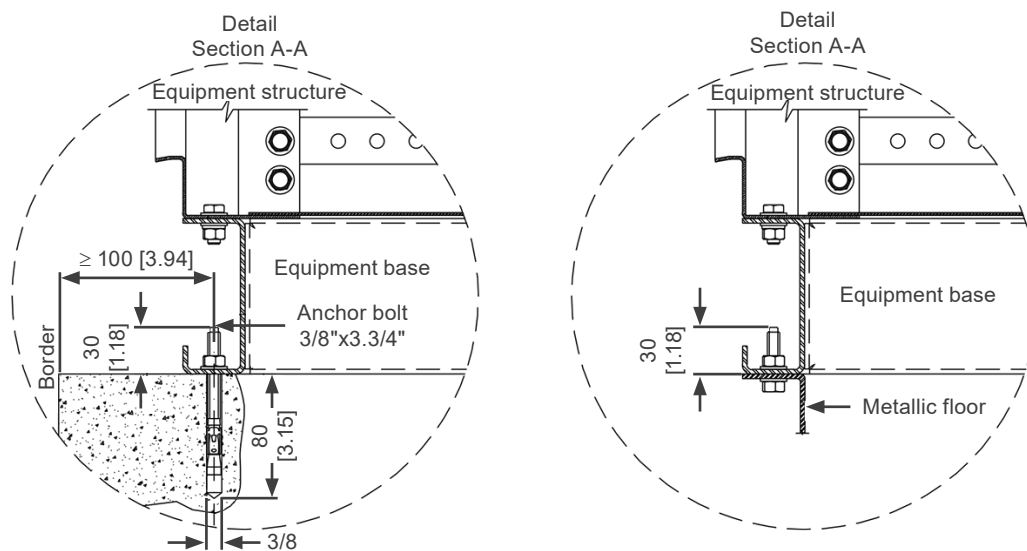
Figure 4.1: Details of the fastening of the panels to concrete floor and metal floor
