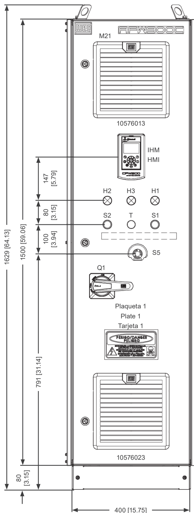
Figure 4.7: Mechanical details of frames C and D
