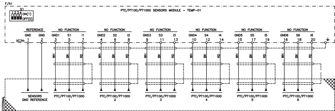
Figure 2.7: TEMP-01 electrical connection
