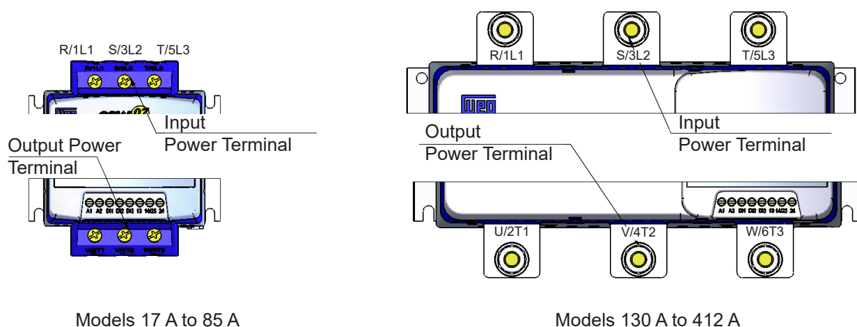
Figure 3.5 - Power terminals
