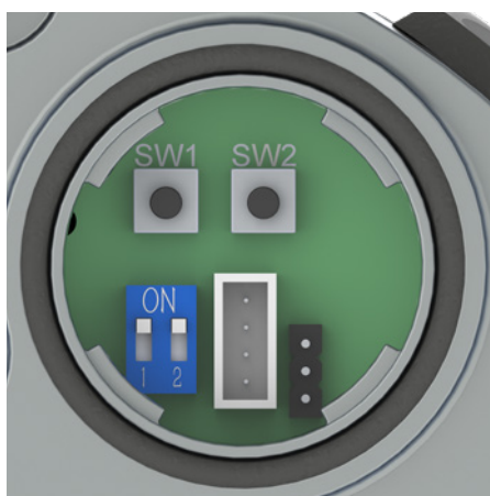
Figure 6.1: Product standard control switches
