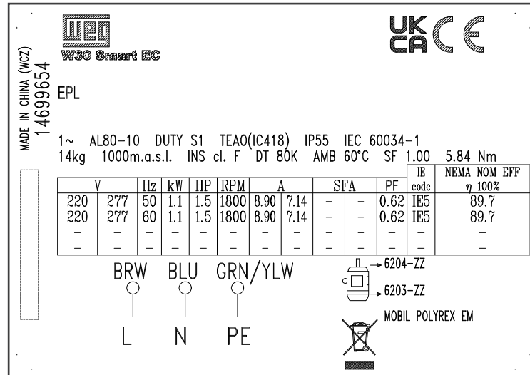
Figure 4.1: Motor nameplate for IEC80 frame
