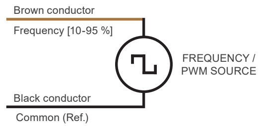
Figure 7.6: Frequency input
