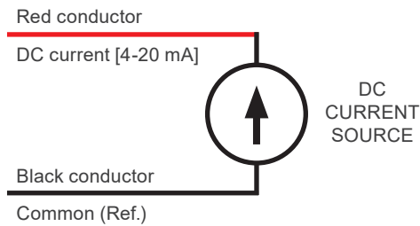
Figure 7.5: DC current input
