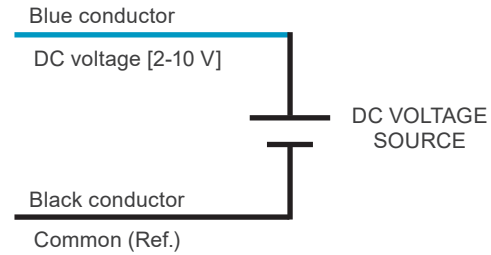
Figure 7.7: DC voltage input (using external power supply)
