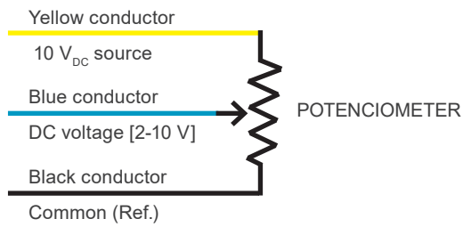
Figure 7.4: DC voltage input (using built-in power supply)
