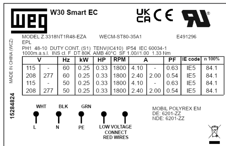
Figure 4.2: Motor label identification for Nema 48 frame
