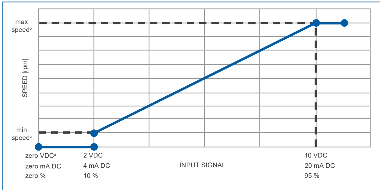
Figure 7.8: Control input reference
