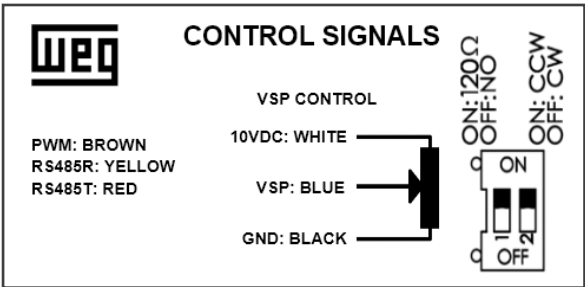
Figure 7.2: Signal cables functions label, for Modbus version
