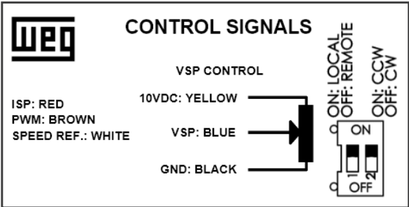
Figure 7.1: Signal cables functions label, for standard version
