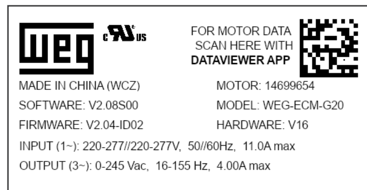
Figure 4.3: Drive label
