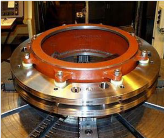
Hub & Split Collector Ring Assembly
