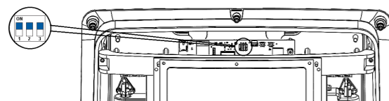
Figure 5.1: Rated current selection switches
