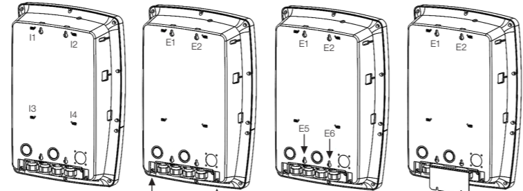
Figure 4.2: WEMOB-PARKING mounting methods
