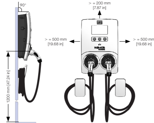
Figure 4.1: Mounting position and spacing of the WEMOB-PARKING
