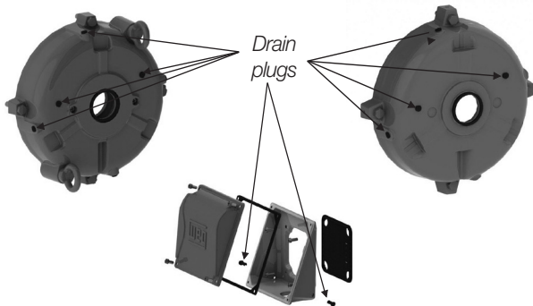
Drain plugs positions
