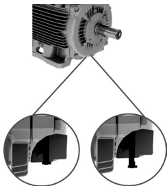
Drain plug closed Drain plug open
