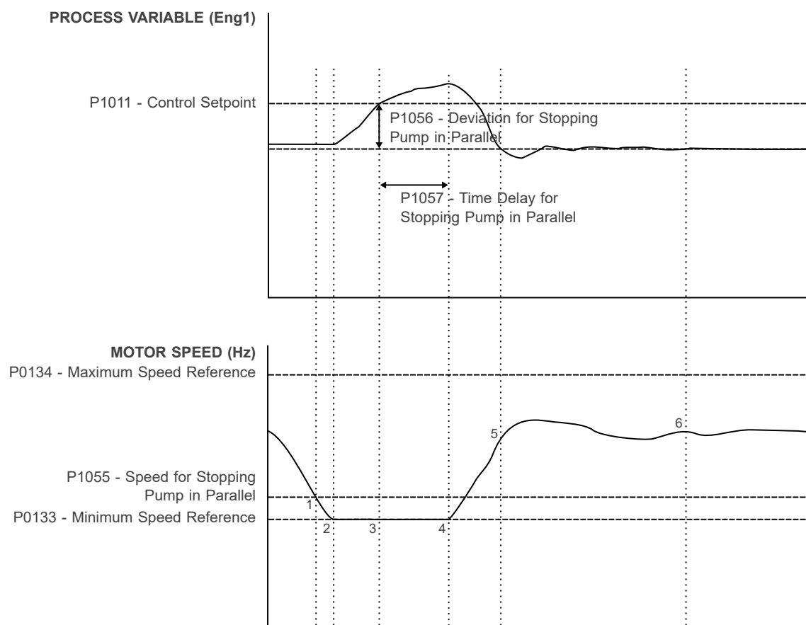
Figure 5.8: Pump Genius Multiplex operation for stop one pump in parallel
