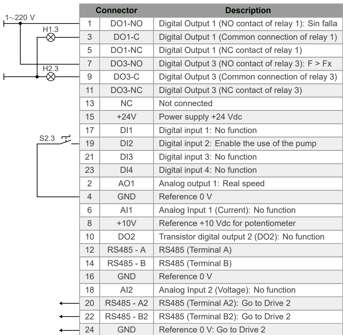
Figure 4.40: Signals on connector of the CFW500-RS485 plug-in module for slave pump (Pump 3)
