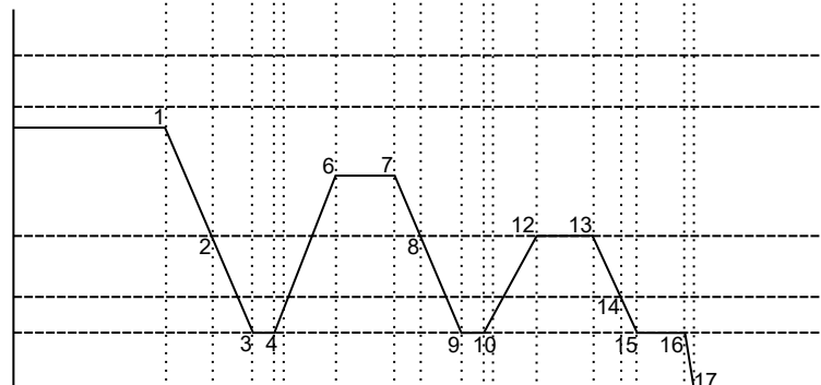
Figure 4.36: Operation description of the Pump Genius Multiplex with three pumps in parallel
