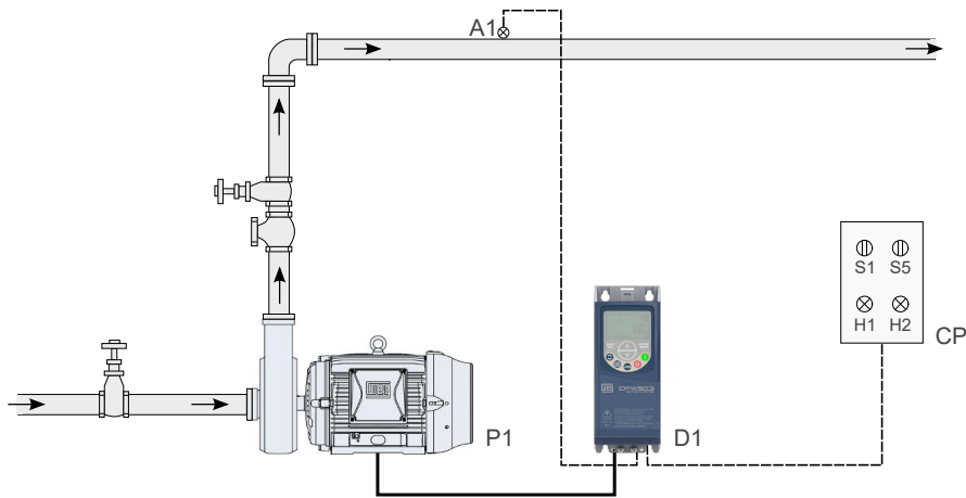
Figure 4.7: Pump Genius Simplex application and selection of PID controller in manual or automatic via digital input DI3
