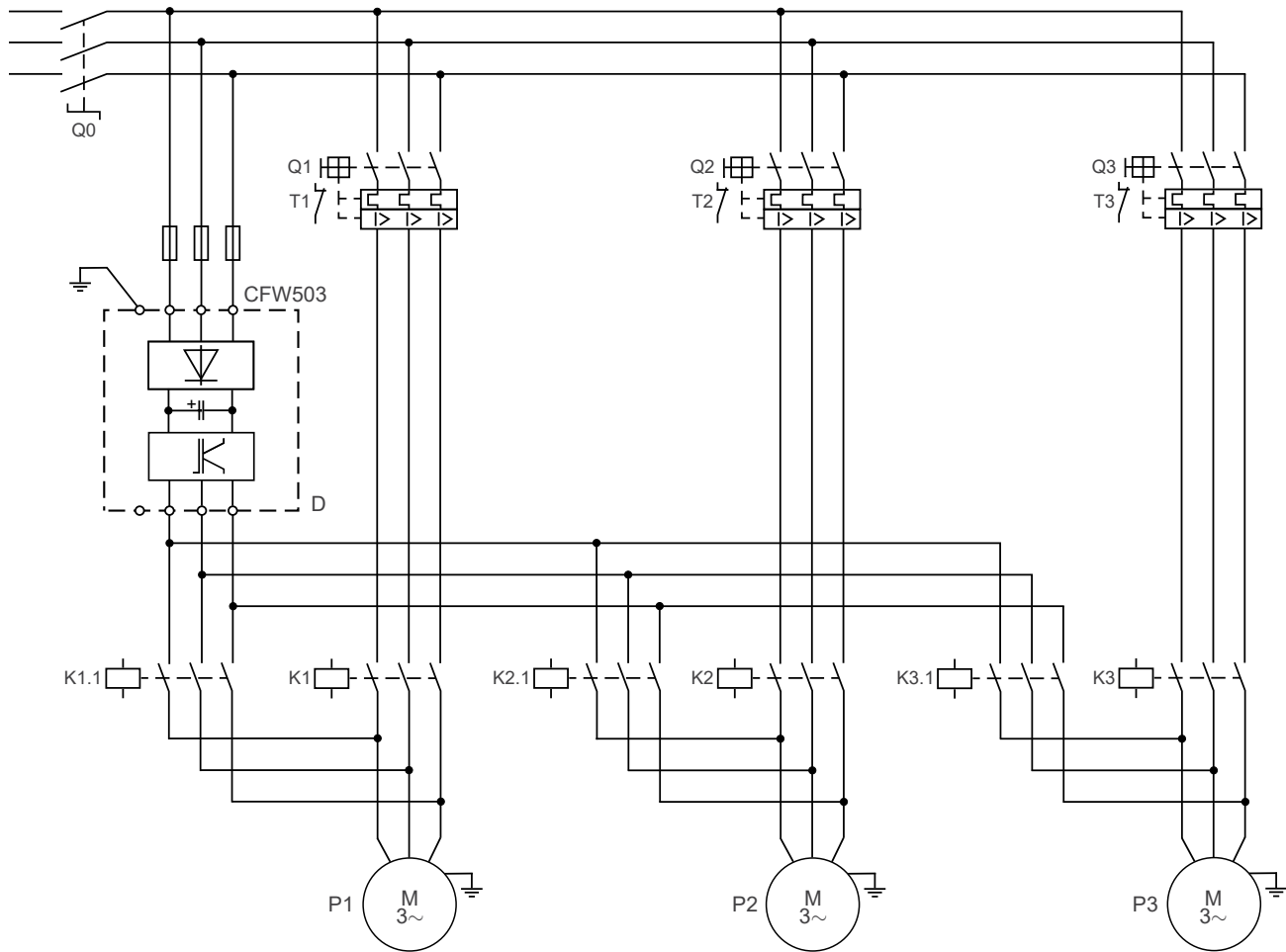
Figure 4.22: Power connections of the Pump Genius Multipump application with floating control and three pumps in parallel
