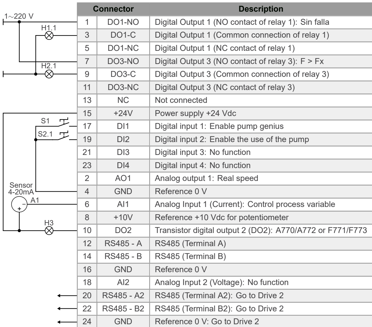
Figure 4.31: Signals on connector of the CFW500-RS485 plug-in module for master/slave pump (Pump 1)
