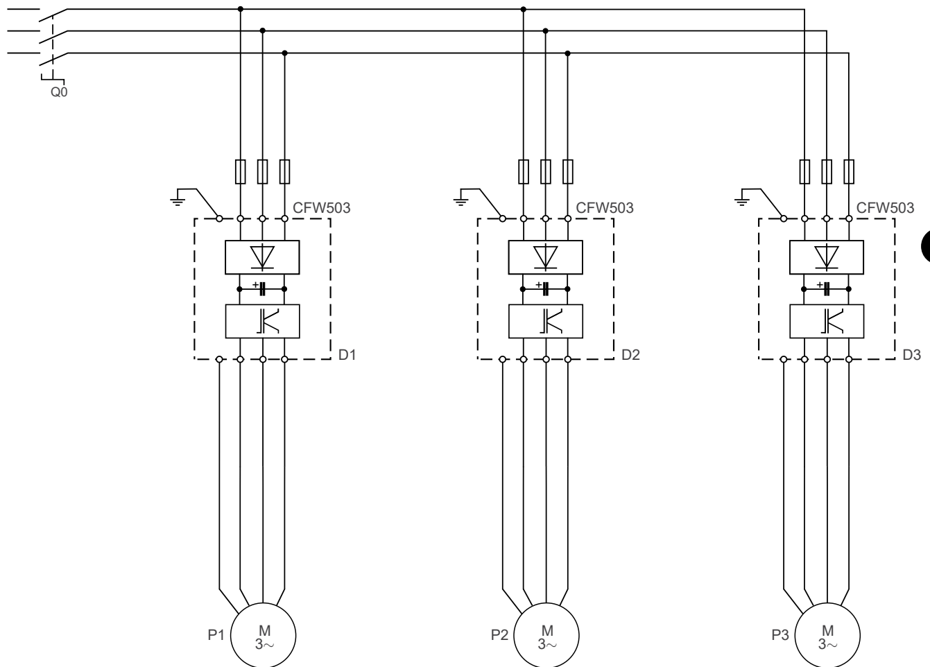
Figure 4.41: Power connections of the Pump Genius Multiplex application with three pumps in parallel
