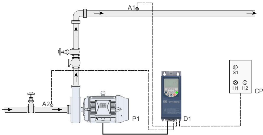
Figure 4.11: Pump Genius Simplex application and pump protection via control auxiliary variable read by analog input
