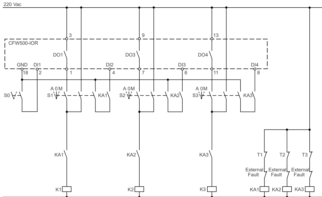
Figure 4.18: Command connections of the Pump Genius Multipump application with fixed control and four pumps in parallel
