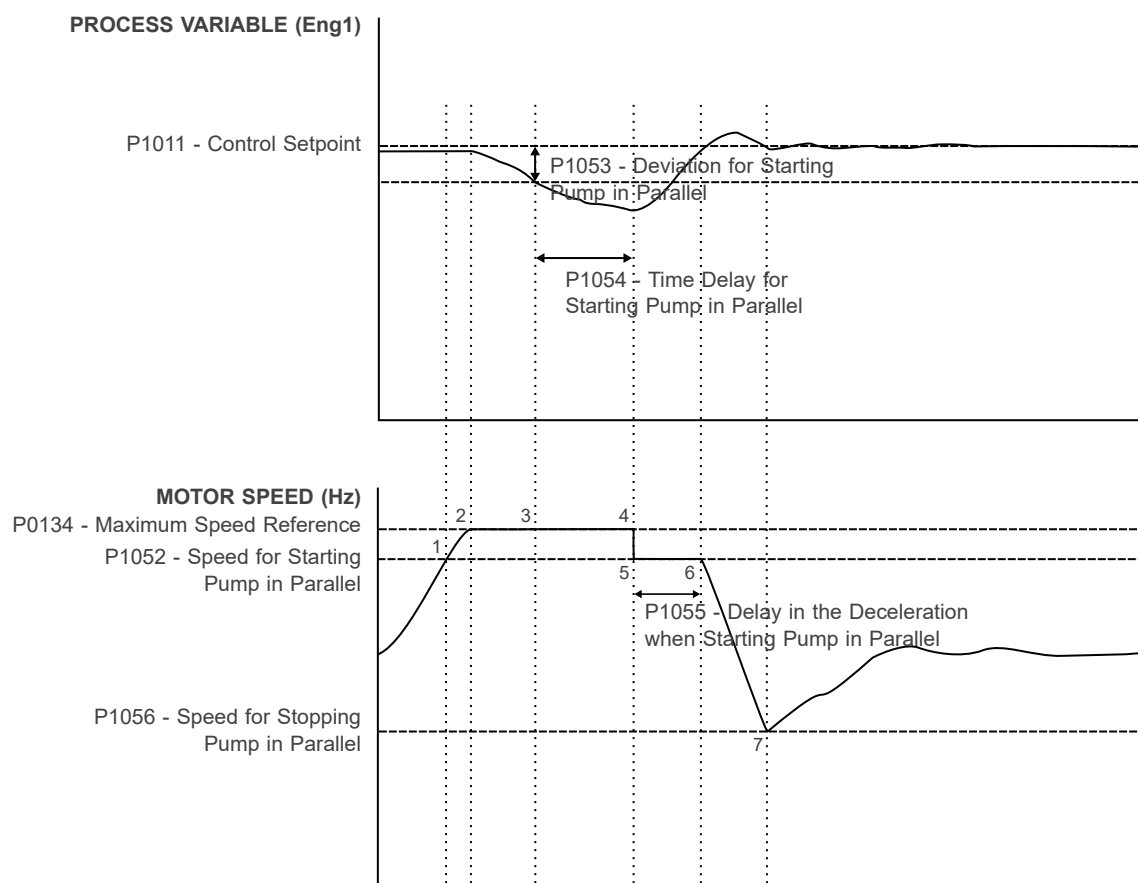
Figure 5.5: Pump Genius Multipump operation for starting an additional pump in parallel
