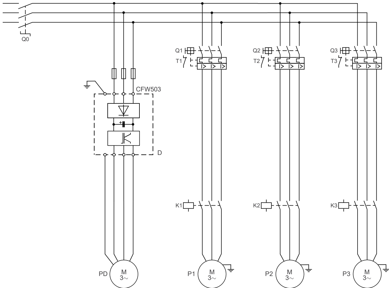
Figure 4.17: Power connections of the Pump Genius Multipump application with fixed control and four pumps in parallel
