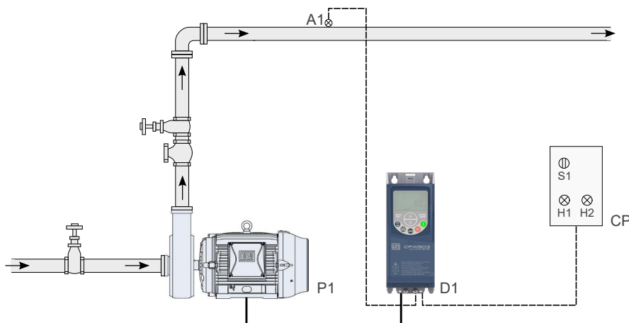
Figure 4.1: Pump Genius Simplex application and control setpoint via HMI
