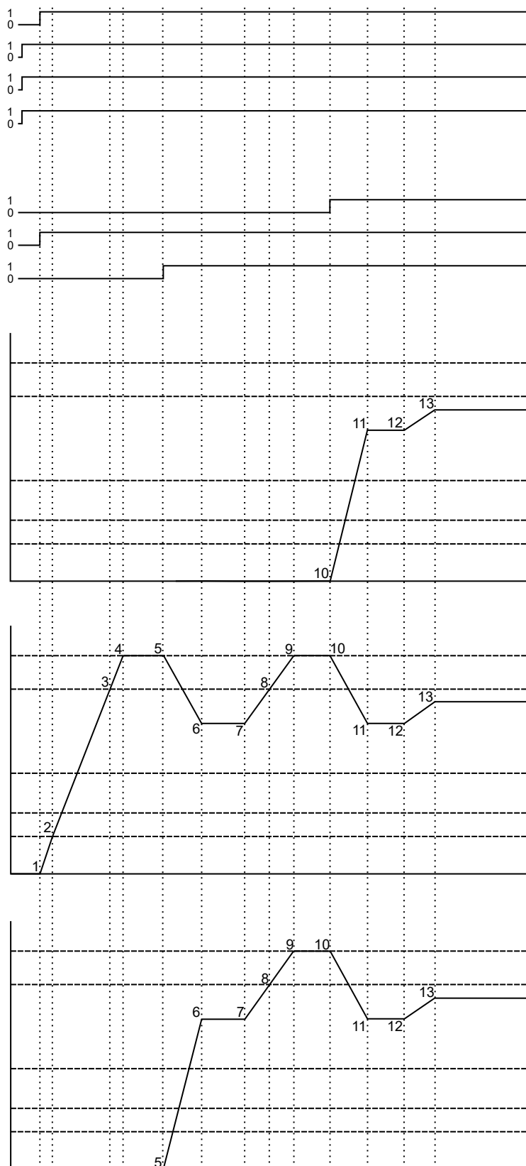
Figure 4.42: Operation description of the Pump Genius Multiplex with three pumps in parallel
