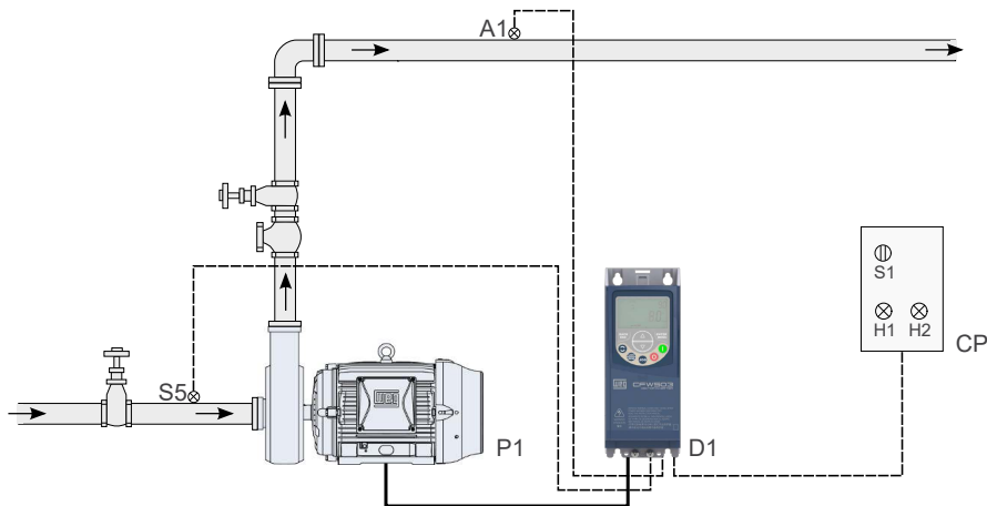
Figure 4.9: Pump Genius Simplex application and pump protection via external sensor in the digital input DI1
