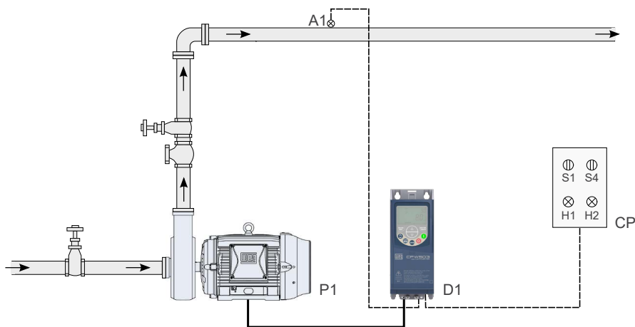
Figure 4.5: Pump Genius Simplex application and control setpoint via combination of the digital inputs DI4 and DI5
