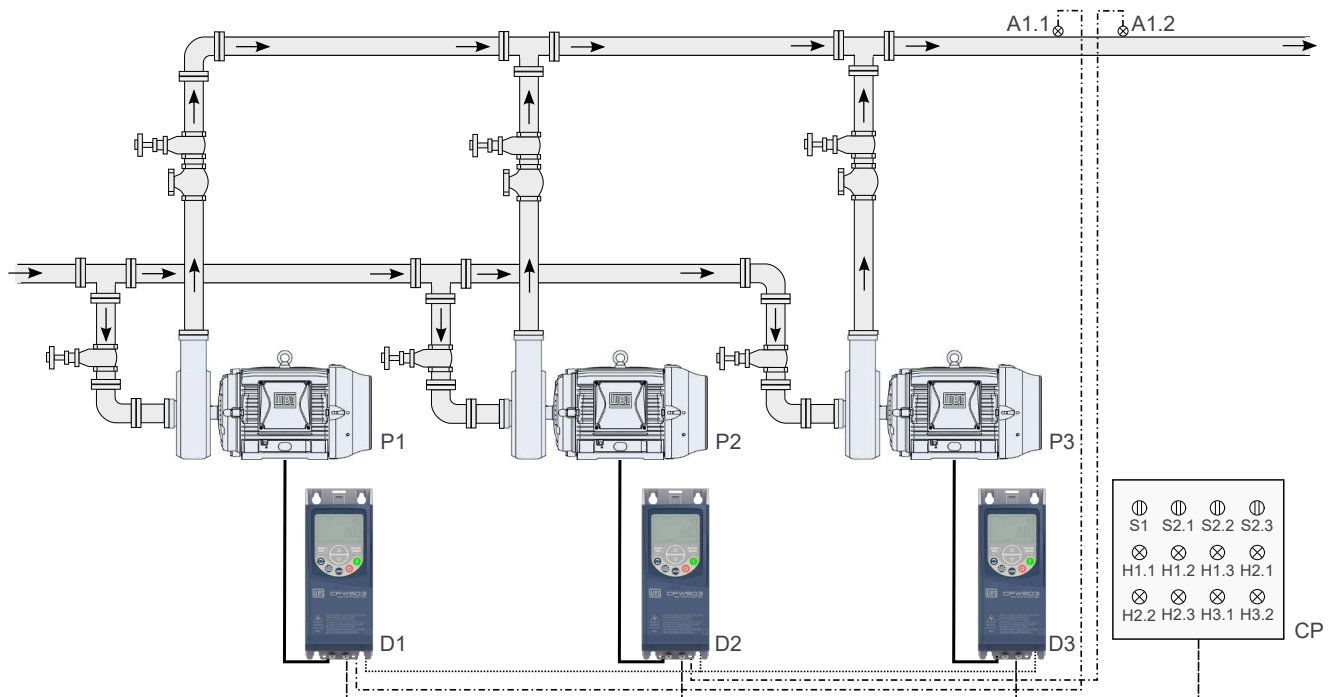
Figure 4.37: Pump Genius Multiplex application with 2 master/slave pumps and one slave pump in parallel and RS485 communication interface
