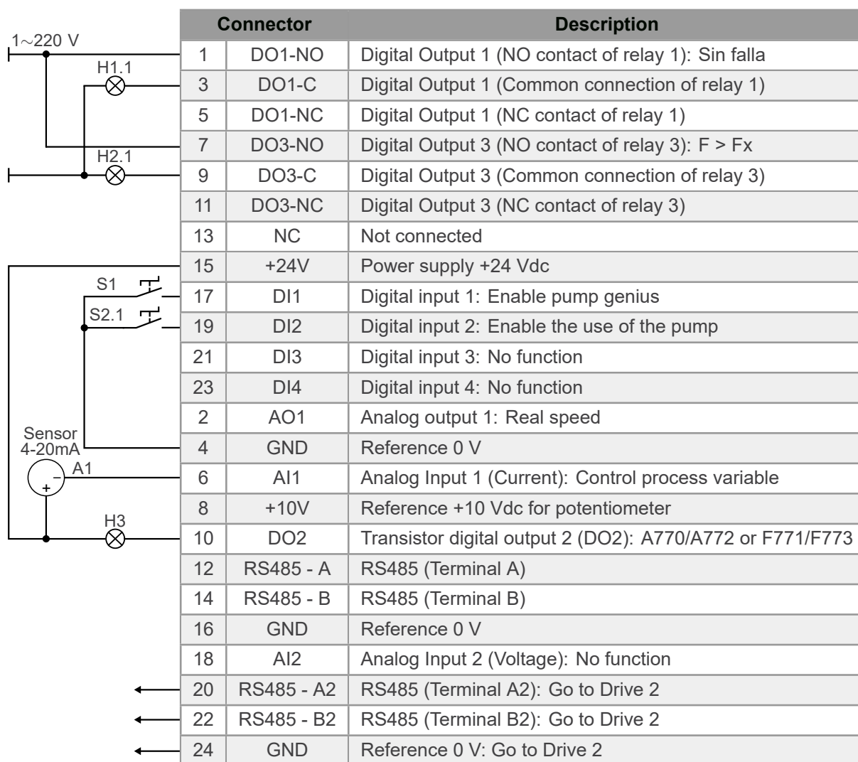
Figure 4.26: Signals on connector of the CFW500-RS485 plug-in module for master/slave pump (Pump 1)
