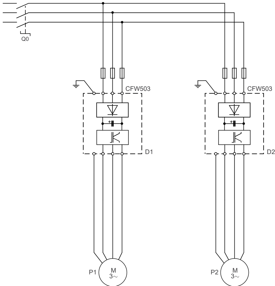
Figure 4.28: Power connections of the Pump Genius Multiplex application with two pumps in parallel
