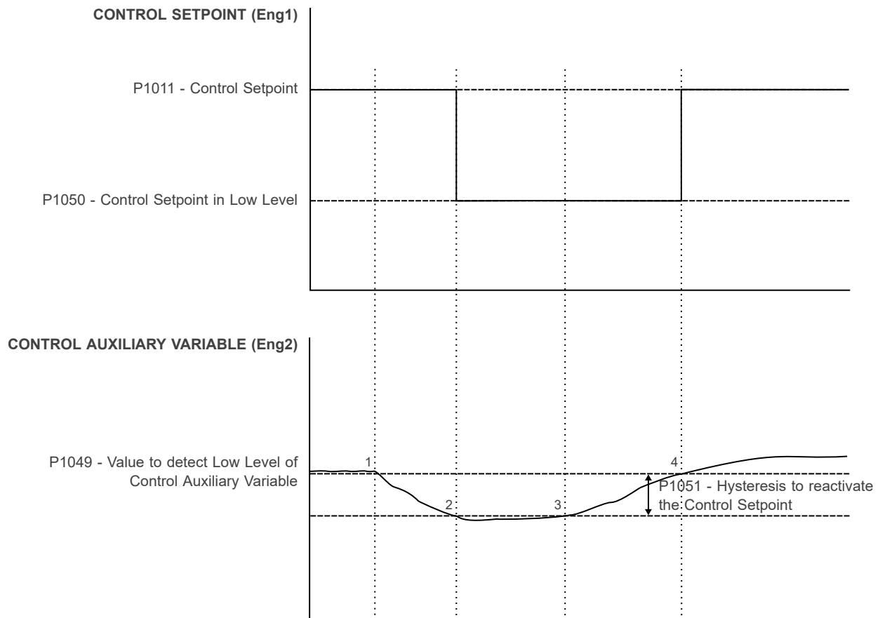
Figure 5.10: Pump Genius operation with pump protection via control auxiliary variable
