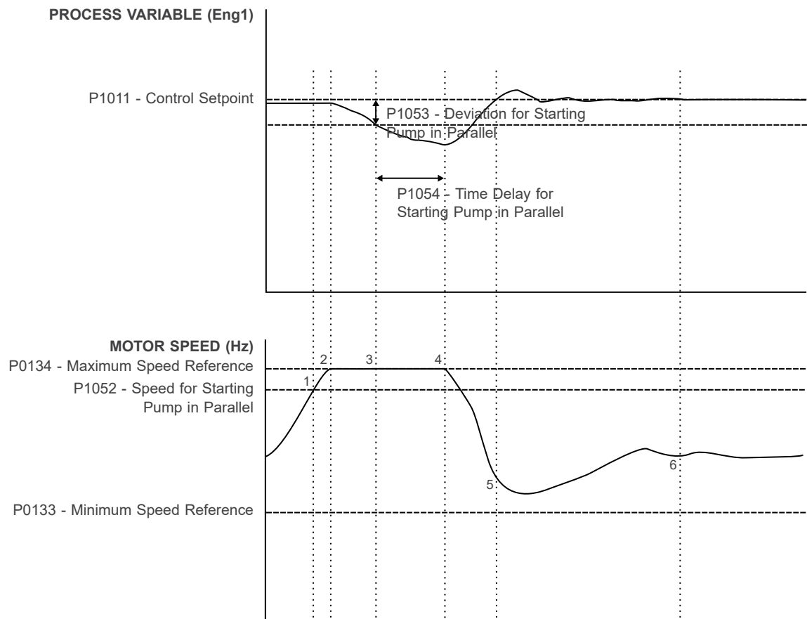
Figure 5.6: Pump Genius Multiplex operation for starting an additional pump in parallel
