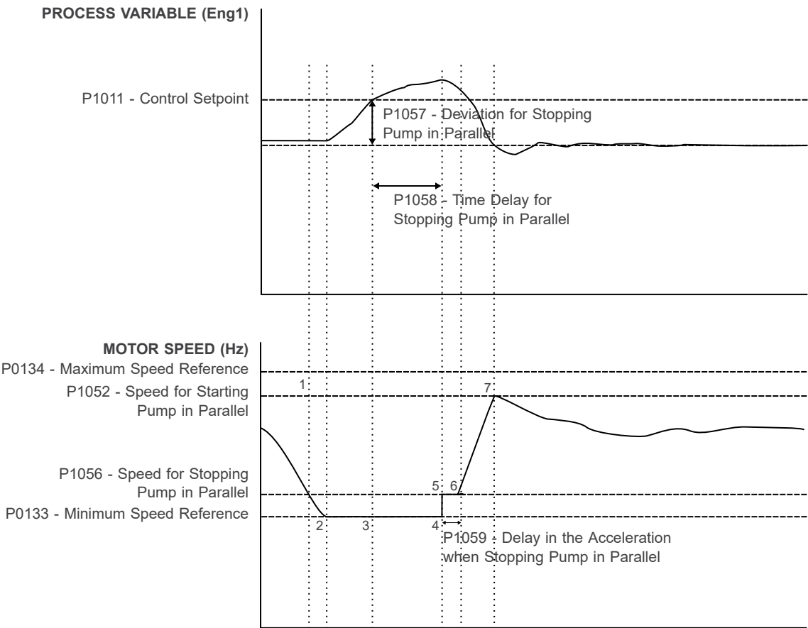
Figure 5.7: Pump Genius Multipump operation for stop one pump in parallel
