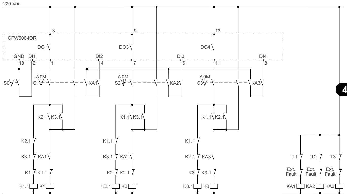
Figure 4.23: Command connections of the Pump Genius Multipump application with floating control and three pumps in parallel
