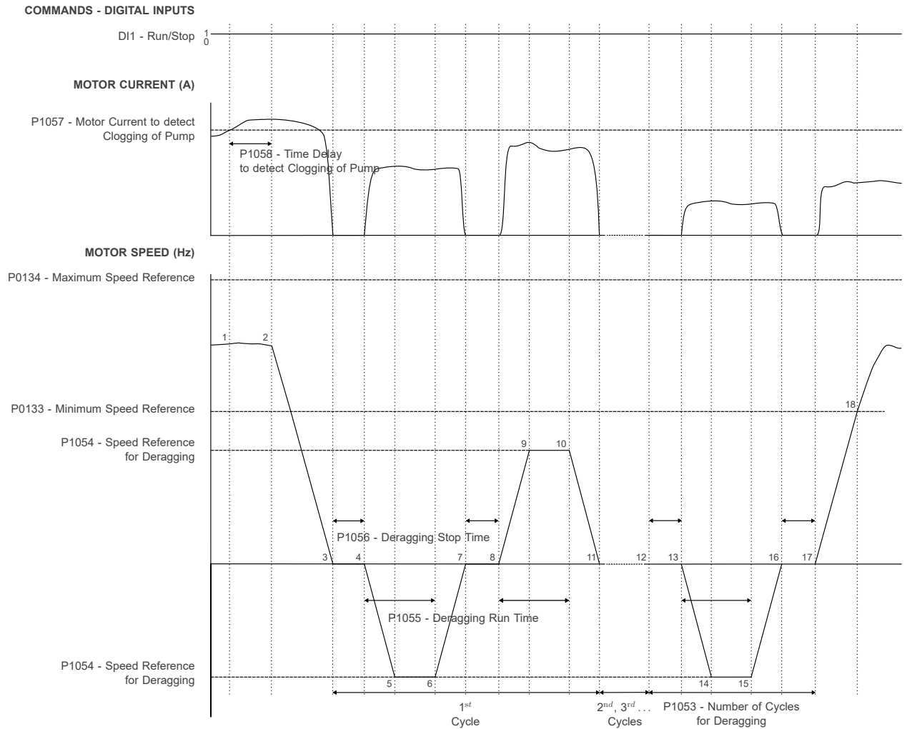
Figure 5.13: Deragging pump operation when a clogging of pump is detected
