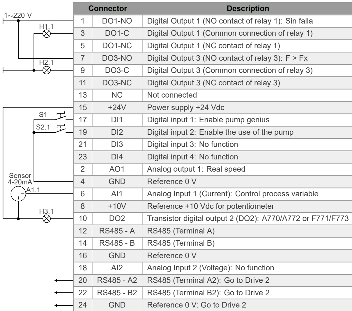
Figure 4.38: Signals on connector of the CFW500-RS485 plug-in module for master/slave pump (Pump 1)
