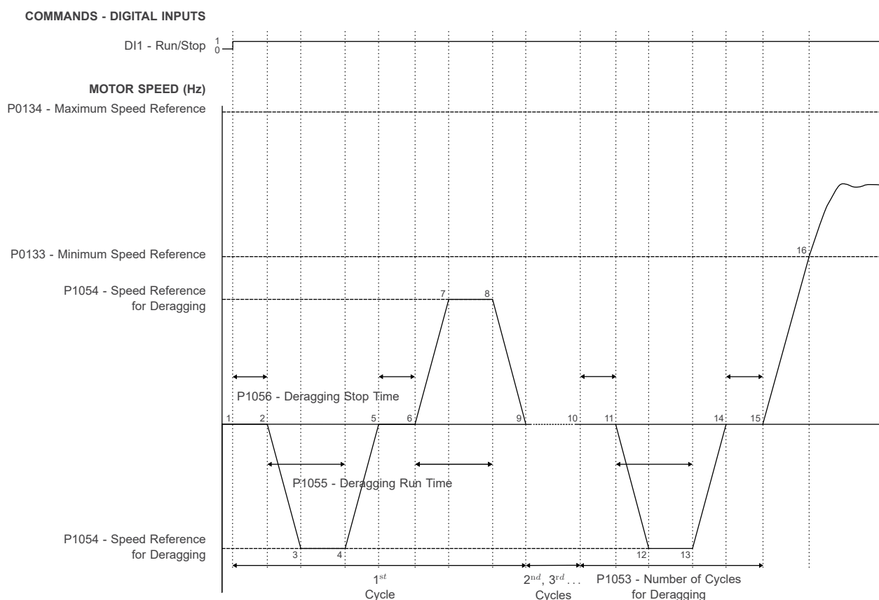
Figure 5.11: Deragging pump operation with command to run the pump
