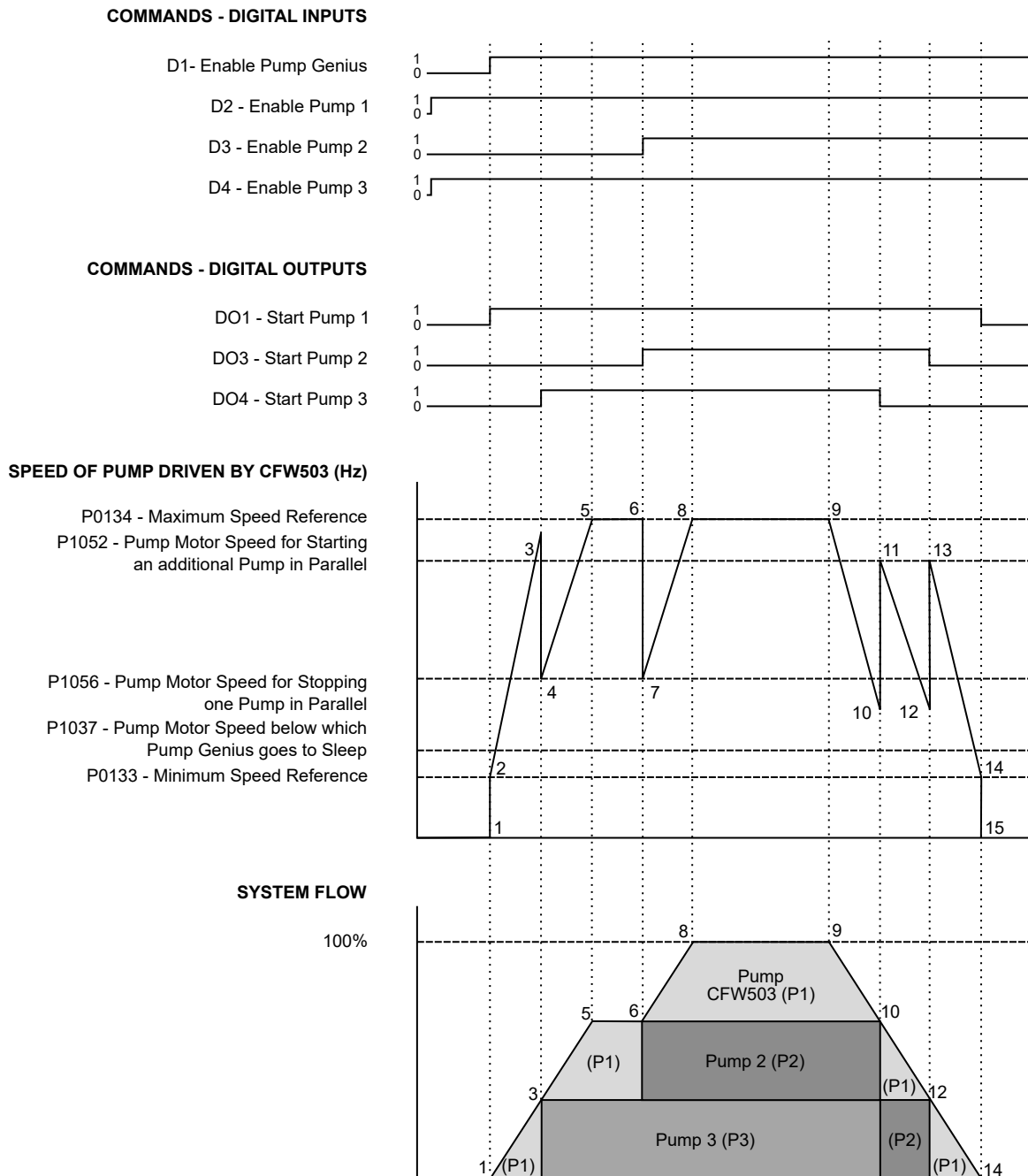
Figure 4.24: Operation description of the Pump Genius for floating control
