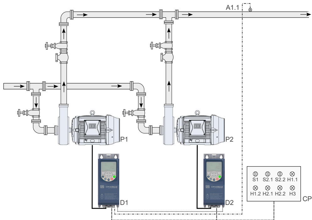
Figure 4.25: Pump Genius Multiplex application with two pumps in parallel and RS485 communication interface
