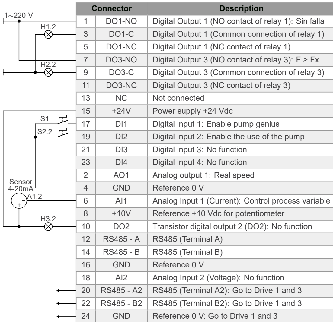
Figure 4.39: Signals on connector of the CFW500-RS485 plug-in module for master/slave pump (Pump 2)
