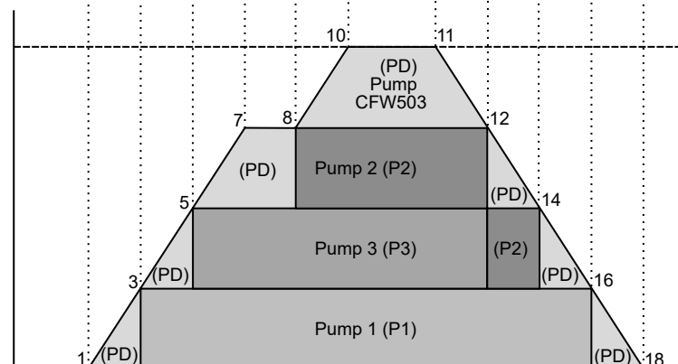
Figure 4.19: Operation description of the Pump Genius for fixed control
