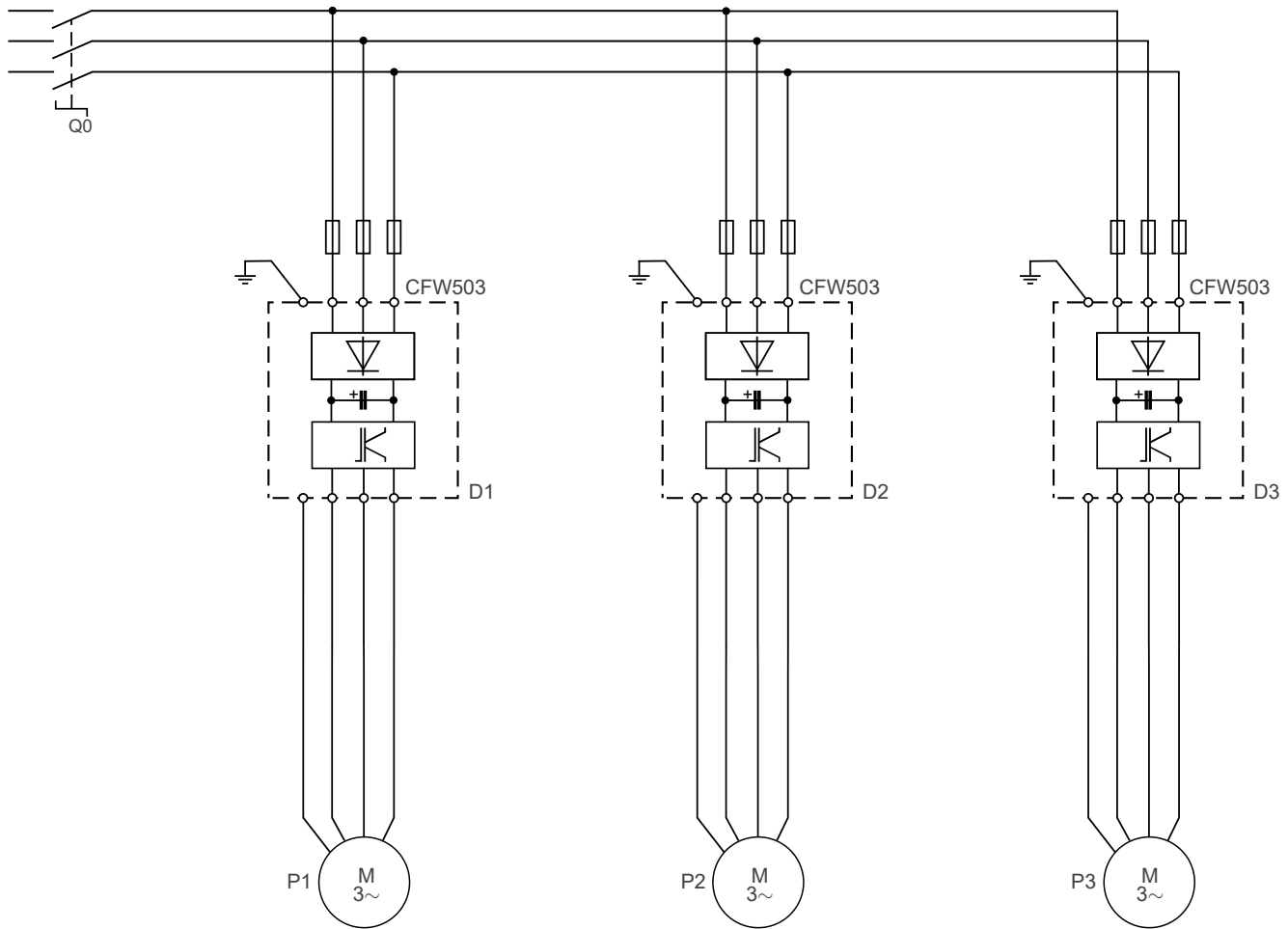
Figure 4.34: Power connections of the Pump Genius Multiplex application with three pumps in parallel
