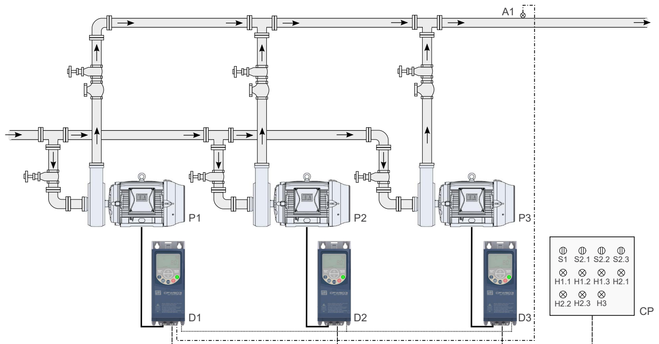
Figure 4.30: Pump Genius Multiplex application with 1 master Pump and two slave pumps in parallel and RS485 communication interface
