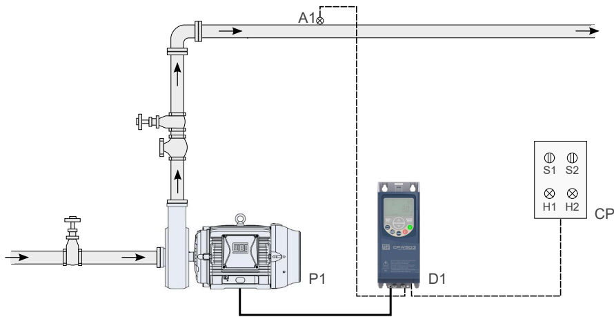
Figure 4.13: Pump Genius Simplex application and deragging function with command via digital input DI2
