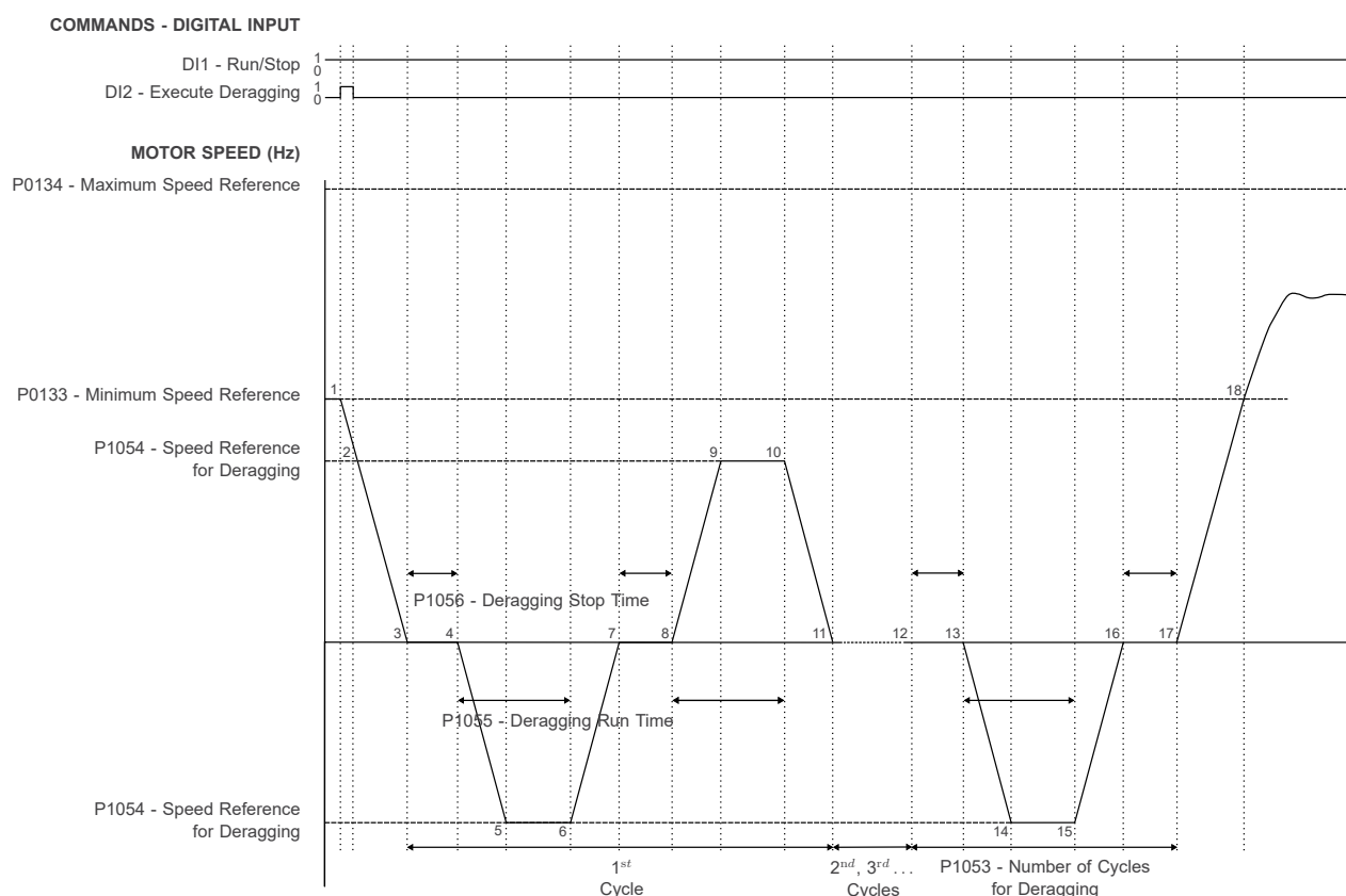
Figure 5.12: Deragging pump operation with command via digital input DI2
