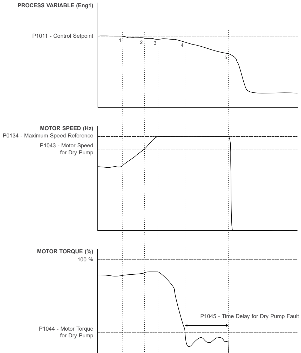
Figure 5.9: Operation of the Pump Genius for dry pump protection
