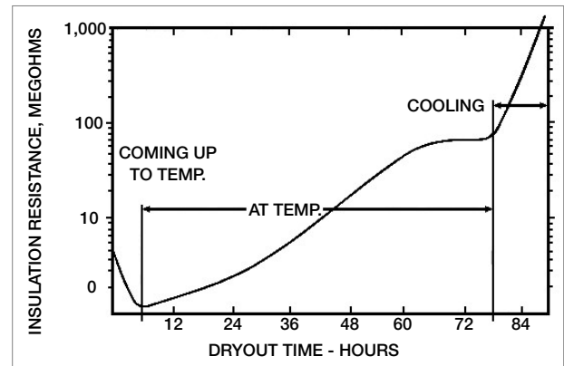
Figure 7-4: Typical Drying Out Curve
