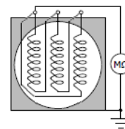
Figure 7-1: Connection of the Megohmmeter to the Stator Winding
