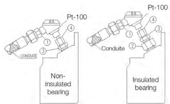
Figure 17-9: Pt100 on the Bearings
