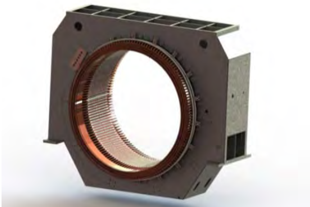
Figure 8-2: Stator
