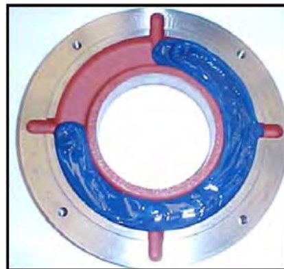
Figure 17-8: External Bearing Cap
