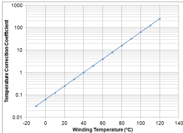
Figure 7-3: Plot of Temperature Correction Coefficient verses Winding Temperature.
