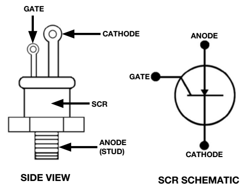
Figure 17-2: SCR Connections
