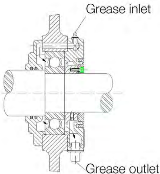
Figure 17-10: Grease-Filled Rolling Element Bearings
