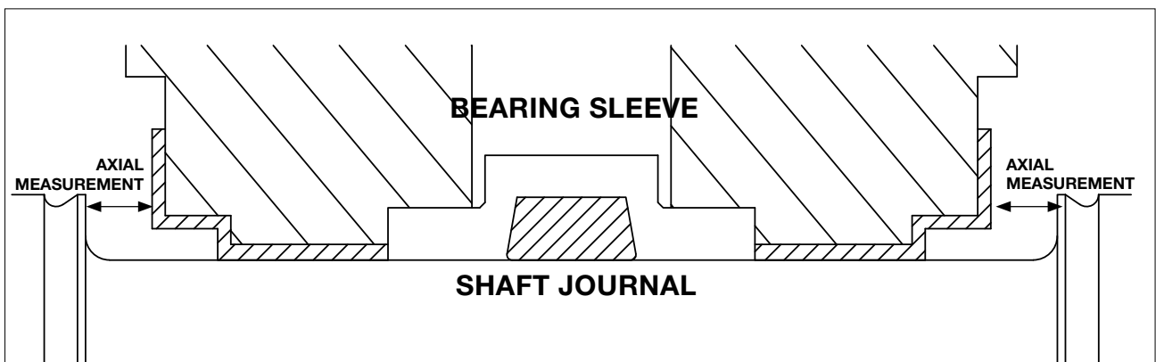
Figure 10-3: Bearing Mechanical Center
