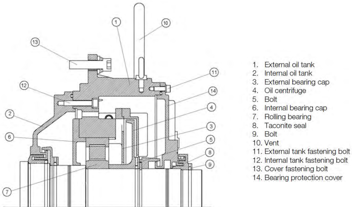
Figure 17-6: Parts of the Oil-Filled Rolling Element Bearing
