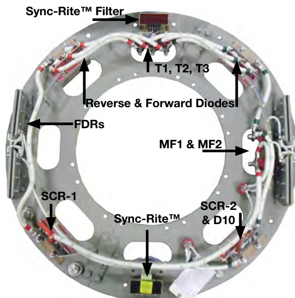
Figure 17-1: Typical Diode Wheel
