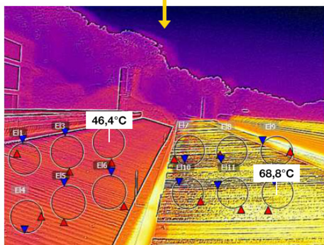
Figure 01: The Thermal Analysis Report shows the temperature difference between a coated and an uncoated roof. Images captured with the Flir One Pro thermographic camera.
