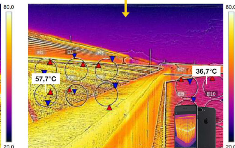
Figure 01: The Thermal Analysis Report shows the temperature difference between a coated and an uncoated roof. Images captured with the Flir One Pro thermographic camera.
