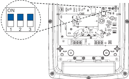
Figure 5.1: Rated current selection switches
