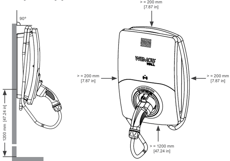
Figure 4.1: Mounting position and spacing of the WEMOB-WALL
