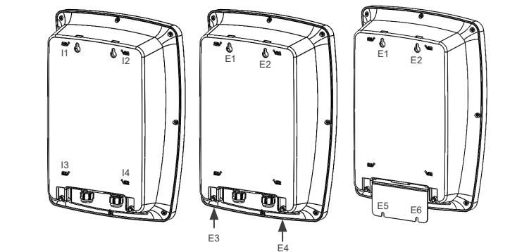
Figure 4.2: WEMOB-WALL mounting methods
