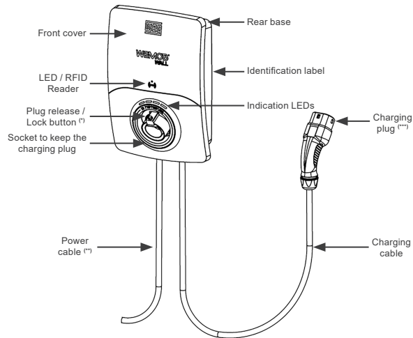
Figure 2.1: WEMOB-WALL overview
