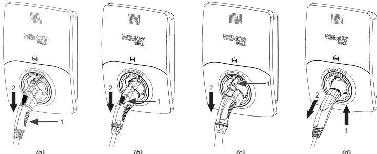
Figure 5.4: (a), (b), (c) and (d) Procedure for removing the plug from the socket on charging stations with cables type 1, GB/T, type 2 and NACS
