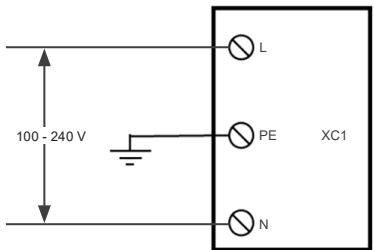
Figure 5.2: Internal electrical connection
