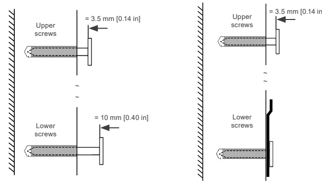
(a) Mounting without the metal bracket
