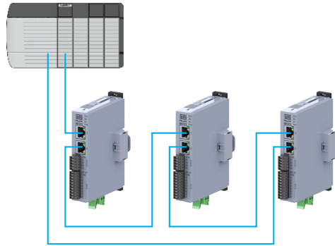
Figure 3.4: Ring topology
