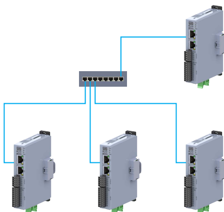
Figure 3.2: Star topology
