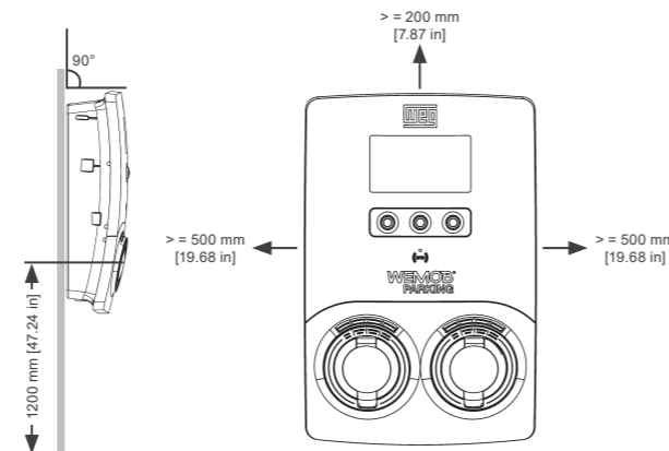
Figure 4.1: Mounting position and spacing of the WEMOB-PARKING 2S2
