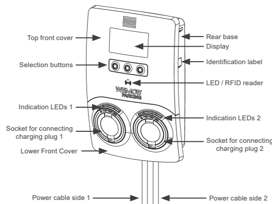
Figure 2.1: WEMOB-PARKING overview
