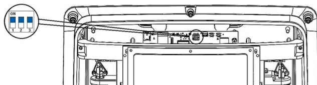
Figure 5.1: Rated current selection switches
