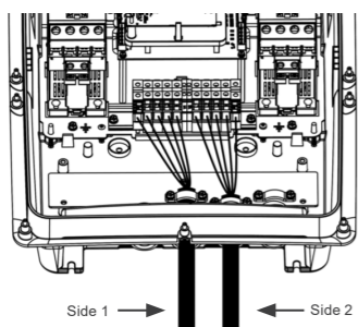
Figure 5.2: Exposed mounting of the power cables (side 1 and 2)
