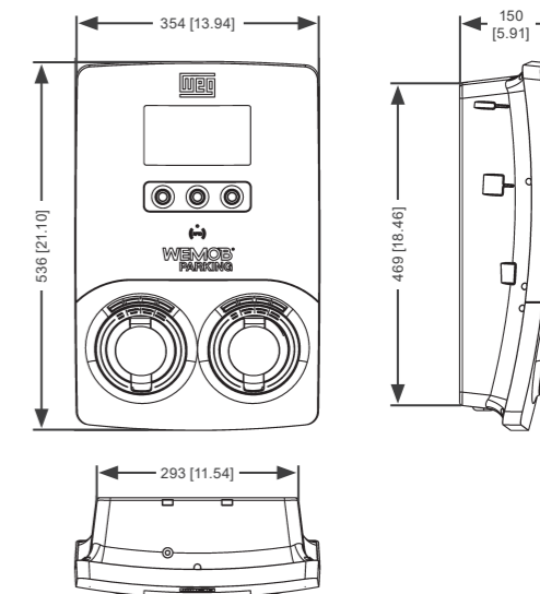
Figure 7.1: Dimensions of the WEMOB-PARKING charging station in mm [in]
