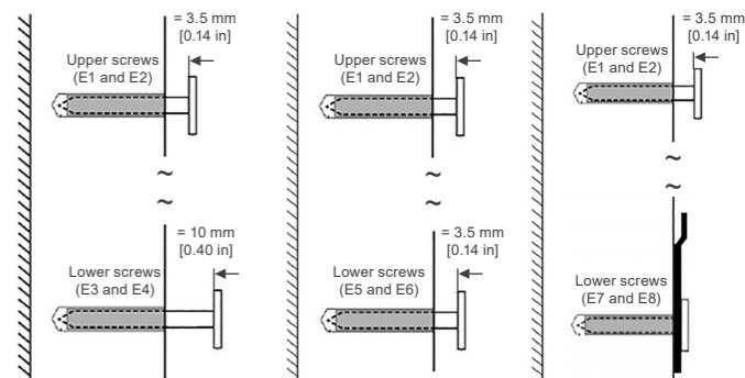
(a) Mounting 1 - without metal bracket (b) Mounting 2 - without metal bracket (c) Mounting with metal bracket
