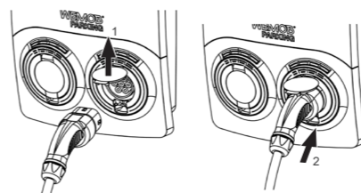
Figure 5.4: Procedure for inserting the plug into the socket
