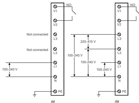
Figure 5.3: Examples of electrical connection: (a) single-phase or two-phase, (b) three-phase
