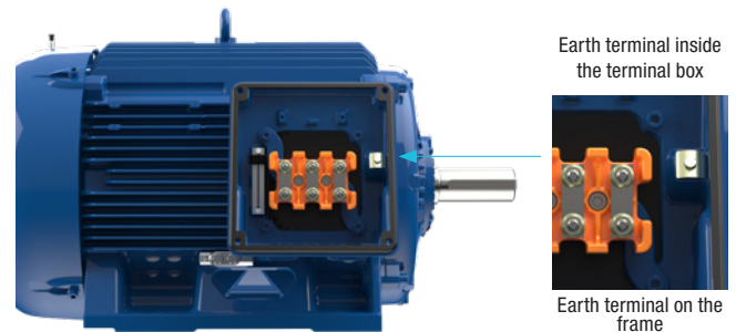
Figure 6. Earth terminal inside the terminal box and on the frame
