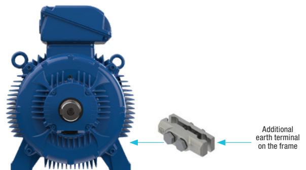
Figure 7. Additional earth terminal position on the frame
