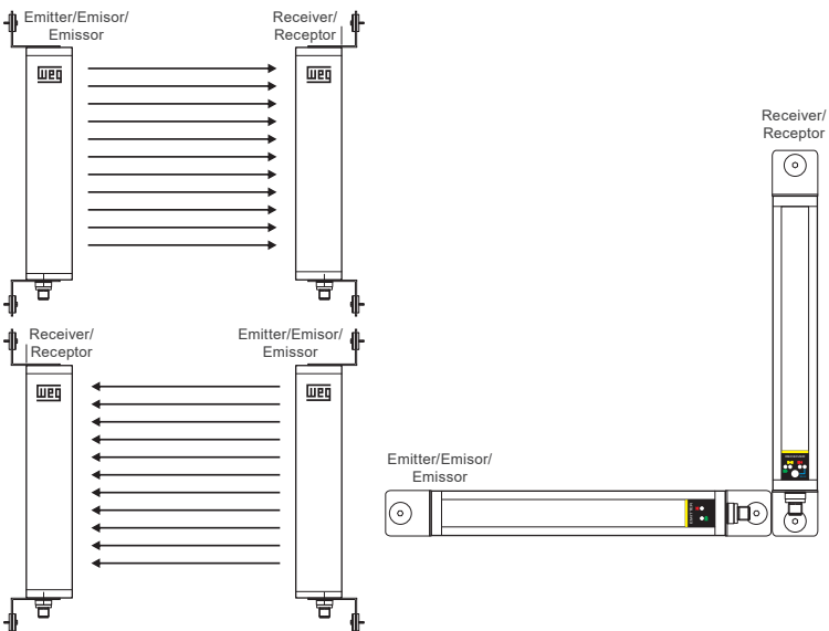
Figure A.4: Emitters in vertical opposite direction and perpendicular alignment
