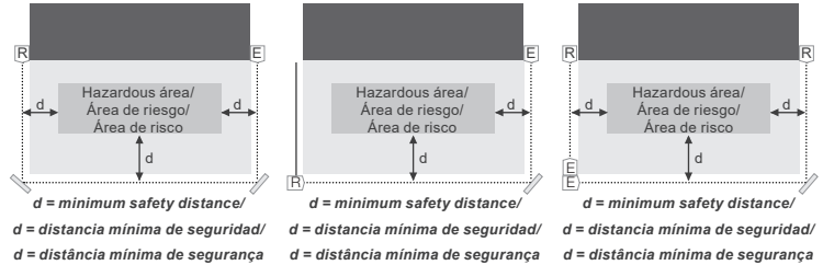
Figure A.5: Examples of applications using mirrors
