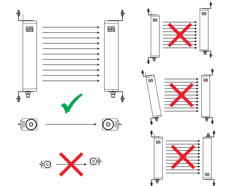
Figure A.2: LGW300 alignment
