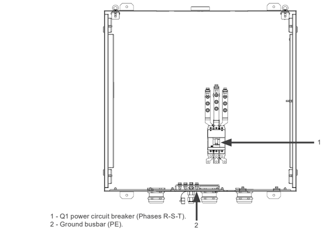
Figure 5.2: Power cable connections - Phases (R-S-T) and ground (PE)
