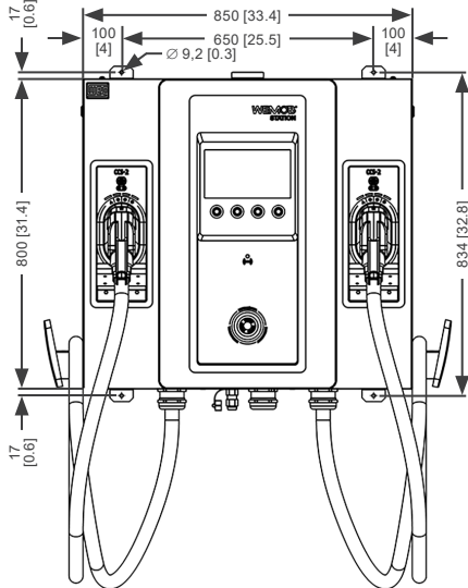
Figure 4.6: Dimensions of the WEMOB-STATION (60/80 kW) for attachment to the concrete structure - mm [in]
