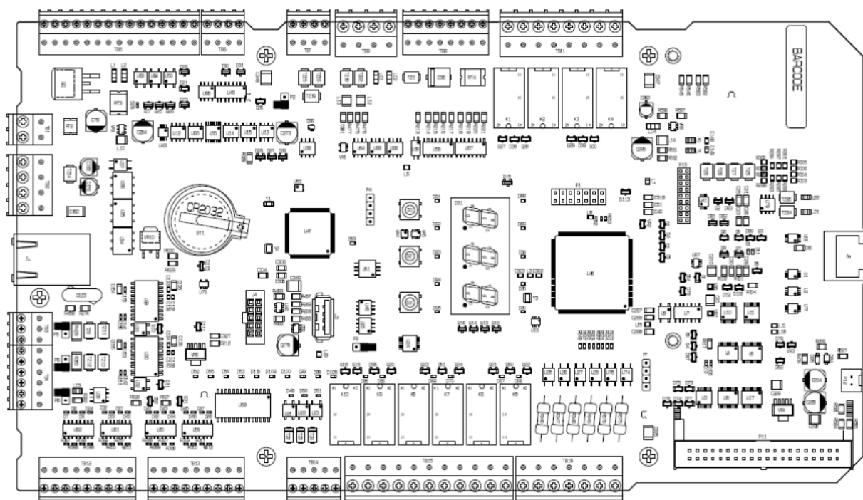
Circuito stampato con componenti ADL550-ICS / Circuit board with components ADL550-ICS
