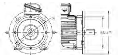
B5 Flange (FF)
