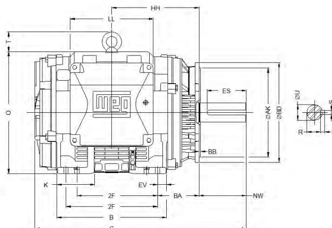
NEMA BA AJ AK BD BF BB BC AH C HH FRAMES NUMBER TAP SIZE 254TC 4.750 7.252 8.500 9.019 4 UNC1/2"-13 0.250 0.250 3.750 21.037 8.876 254/6TC 22.785 8.876 284TC 4,750 9.000 10.500 11.295 5.000 23.158 9.500 284TSC 3.000 21.783 284/6TC 4.375 24.658 10.250 284/6TSC 3.000 23.283 324TC 5.250 11.000 12.500 14.023 UNC5/8"-11 5.000 25.807 10.500 324TSC 3.500 24.307 324/6TC 5.000 27.307 11.250 324/6TSC 3.500 25.807 364/5TC 5.875 14.095 8 5.625 29.725 12.000 364/5TSC 3.500 27.600 404/5TC 6.625 7.000 34.100 13.500 404/5TSC 4.000 31.100 444/5TC 7.500 14.000 16.000 18.024 8.250 38.325 15.750 444/5TSC 4.500 34.358
