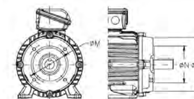
B14 Flange (C-DIN)
