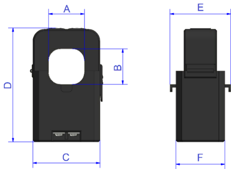
Figura 3 – Sensor Split Core
