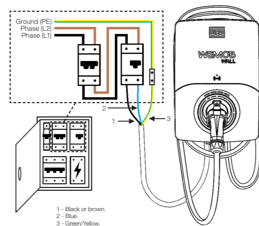
(b) with two-phase circuit breaker and RCD
