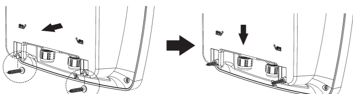
Detail of the lower fitting (screws E3 and E4 -without metal bracket)
