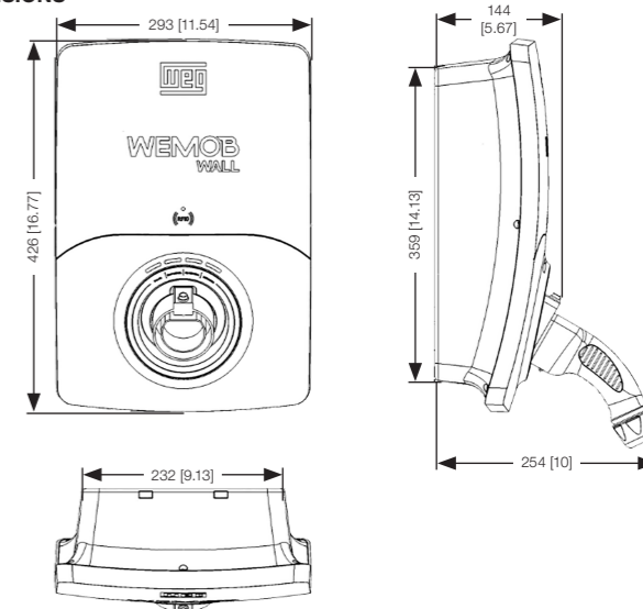
Figure 7.1: Dimensions of the WEMOB-WALL charging station in mm [in]
